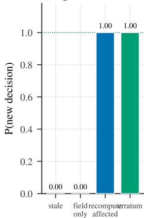
(b) Two fixes recover the ignored edit
