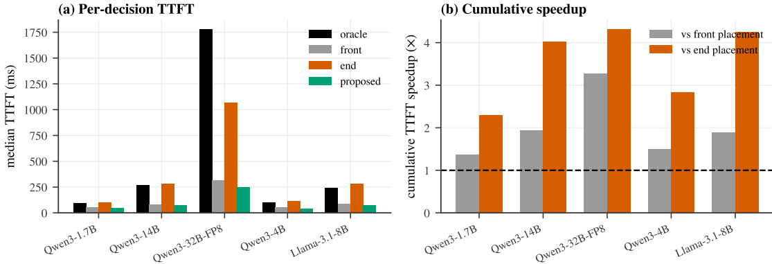
Figure 12: E5 — end-to-end agent. (a) Per-decision median TTFT for the proposed compose+edit agent vs. oracle, front, and end-placement baselines. (b) Cumulative TTFT speedup of 2.3\text{--}4.3\times over refill-every-turn, growing with model size, at faithful next-token decisions.
