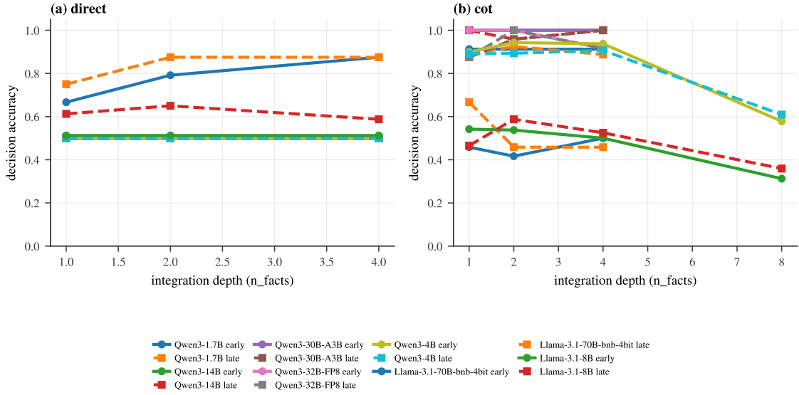
Figure 8: E1 — placement and the pre-digestion cost. Decision accuracy vs. integration depth ( n_{\text{facts}} ) for memory read early (solid) vs. late (dashed), across all evaluated models, under (a) direct answering and (b) chain-of-thought. Direct answering is at chance for the reasoning-native Qwen3 models (so CoT is the operative regime); under CoT, late placement forgoes prefill-time pre-digestion and carries a small accuracy cost vs. early that the text quantifies on Qwen3-4B (GEE-logistic, growing with memory length). Late placement is still preferred because it enables O(L) editing/transplant (efficiency quantified in E5).
