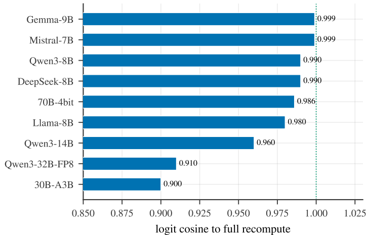
(b) transplant \approx full recompute
