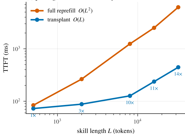
(a) pasting a skill scales linearly
