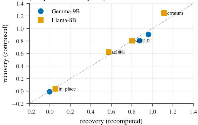
(a) keystone: edit inside a transplant (composed \approx recomputed)
