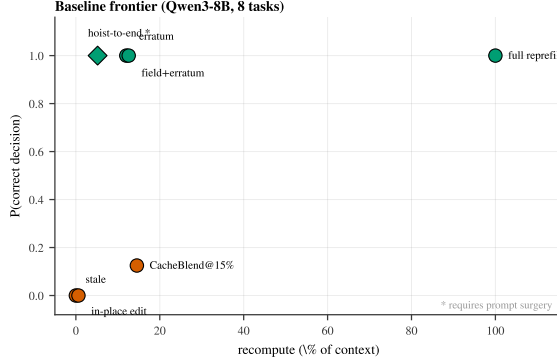
Figure 17: Cost/correctness frontier.
