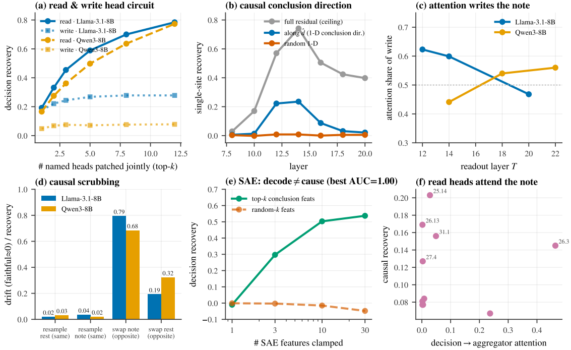
Figure 16: A component-level circuit for memoized inference (Llama-3.1-8B, replicated on Qwen3-8B). (a) Cumulative decision recovery from jointly patching the top- k named read heads (concentrated, \sim 0.78 ) vs. write heads (distributed). (b) A leave-scenario-out difference-of-means conclusion direction causally transfers the decision far above a random 1-D direction. (c) At the causal conclusion layer, attention writes the majority of the note. (d) Causal scrubbing: same-conclusion resampling is faithful (drift \approx 0 ); swapping the note to the opposite conclusion flips the decision while swapping the rest does not. (e) An SAE feature decodes the conclusion perfectly (AUC= 1.0) yet is not causally sufficient alone—the cause is spread over \sim 10 – 30 features. (f) Read heads with the largest causal effect are those that attend decision \rightarrow aggregator.
