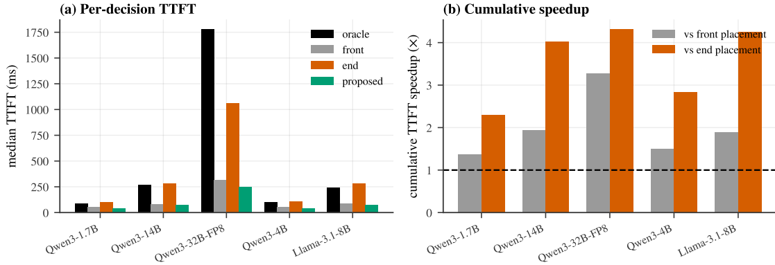
Figure 12: E5 — end-to-end agent. (a) Per-decision median TTFT for the proposed compose+edit agent vs. oracle, front, and end-placement baselines. (b) Cumulative TTFT speedup of 2.3–4.3× over refill-every-turn, growing with model size, at faithful next-token decisions.
