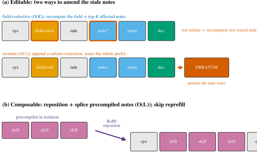
Figure 4: Two cache operations. (a) Editable , two ways to amend the stale notes: field+selective recomputes the field plus the top- K highest-effect downstream notes ( O(K) ; recomputed cells outlined in red, the rest reused stale), while the erratum appends one salient correction ( O(1) , the whole prefix is reused). (b) Composable : precompute a skill’s KV in isolation, RoPE-reposition it to the target positions, and splice it in ( O(L) , no repreload).
