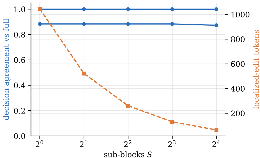
E4: granularity cost/fidelity
