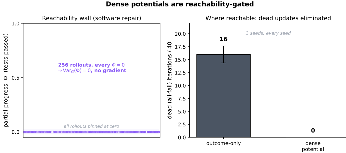
Figure 8. Dense potentials are reachability-gated. Left: on software repair the finer potential is unreachable—across many rollouts the policy makes zero partial progress, so its within-group variance is zero and it gives no gradient. Right: where the potential is reachable, it removes the dead all-fail updates that dominate early outcome-only training (zero versus \sim 16 of 40 iterations, every seed), supplying gradient exactly where the outcome is blind. The gate is reachability, not fragility.
