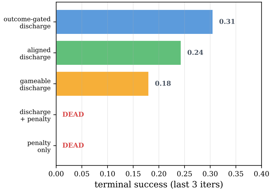
(b) Terminal state: penalty kills, gating rescues
