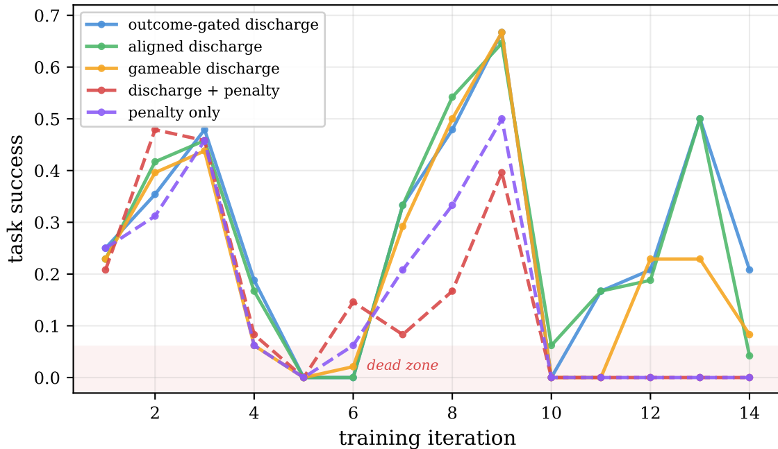
(a) Success trajectory per signal (Qwen3-30B, miniF2F)
