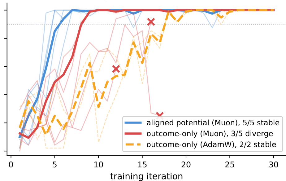
(b) Qwen3-30B-A3B (aligned/Muon 5 seeds; AdamW 2 of 5 done)
