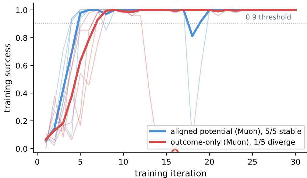
(a) Qwen3-4B, matched optimizer (5 seeds each)
