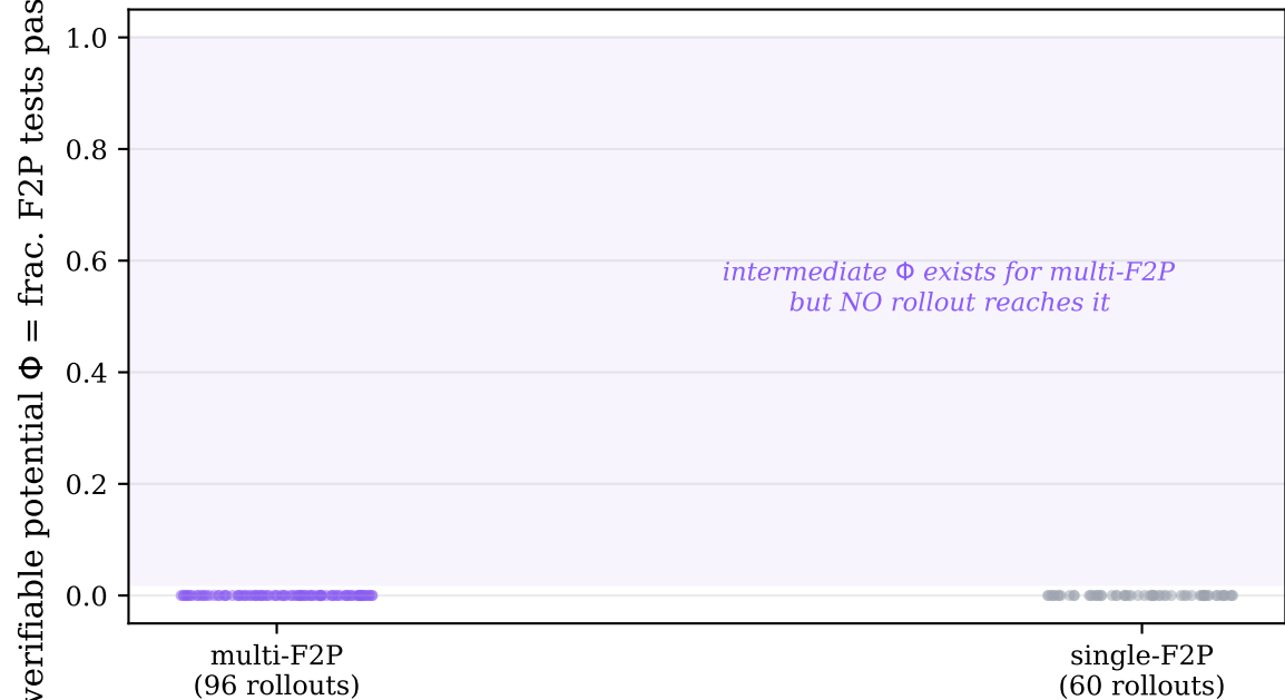
(b) Every rollout sits at \Phi = 0 : the potential is unreachable at 30B
