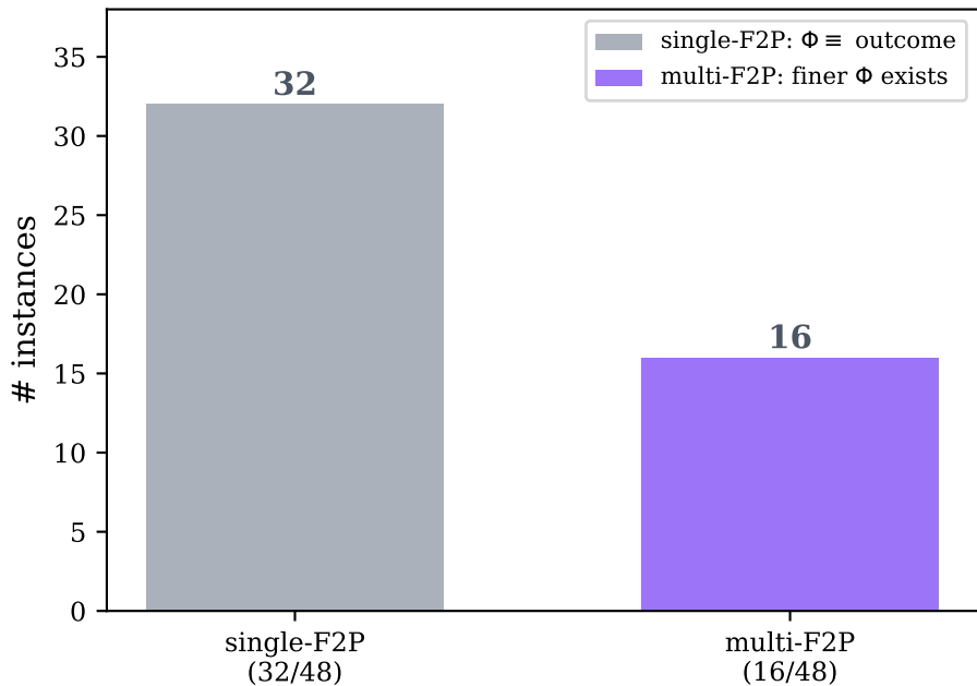
(a) A finer potential is structurally rare: 2/3 are all-or-nothing
