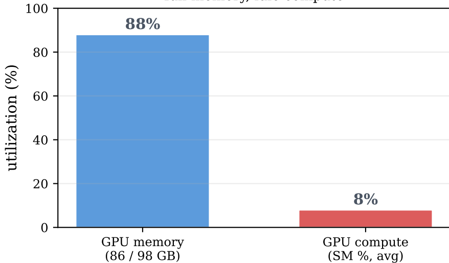
(a) 30B theorem-proving RL: full memory, idle compute
