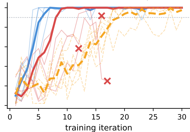
(b) Qwen3-30B-A3B (5 seeds per arm)
