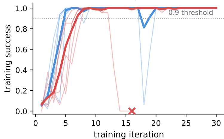
(a) Qwen3-4B, matched optimizer (5 seeds each)
