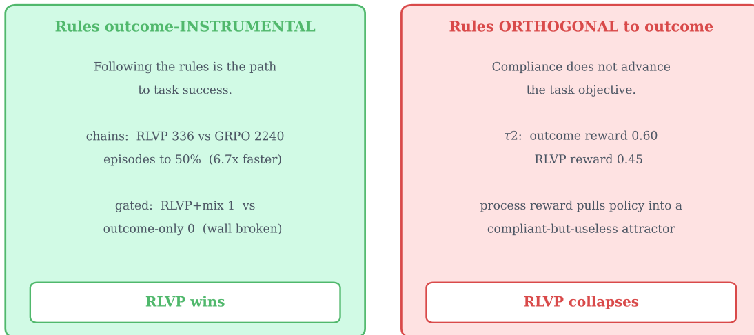
Figure 10. The boundary on a single axis: are the rules outcome-instrumental? When the verifiable rules are aligned with what success requires (chained and gated tasks: the workflow is the task), process rewards convert compliance into large outcome gains. When orthogonal to the reward ( \tau -bench with generic rules), the same machinery optimizes compliance into a degenerate policy.
