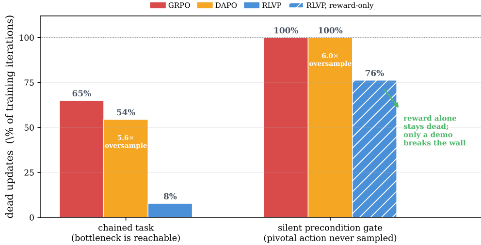
Figure 11. Dead updates across two regimes. Fraction of iterations with an all-fail, zero-spread group (Qwen3-4B, 3-seed mean). Chained task (bottleneck reachable): outcome-only 65%, DAPO 54% at a 5.6\times generation tax, the aligned potential 8%. Silent precondition gate (§A.4, pivotal action never sampled): outcome and DAPO dead on every iteration, the reward-only potential 76%; only a demonstration seed breaks the wall. The cure is a reachable, admissible signal, not density.
