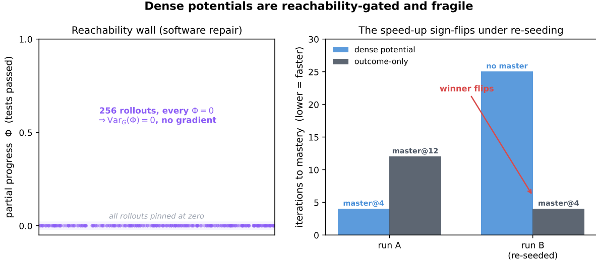
Figure 7. Dense potentials are reachability-gated and fragile. Left: on software repair the finer potential is unreachable—across many rollouts the policy makes zero partial progress, so its within-group variance is zero and it gives no gradient. Right: where a potential is reachable its apparent speed-up does not survive re-seeding—the same configuration reverses sign across runs. The reliable half of the process signal is the penalty, not the potential.
