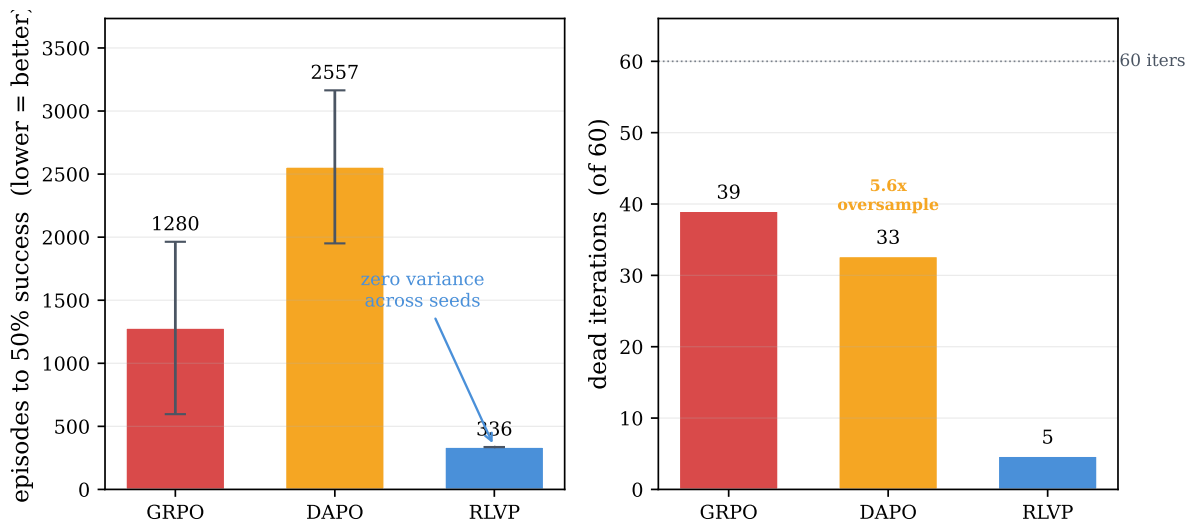
Figure 13. Efficiency over three seeds. Left: episodes to the success threshold (lower better)—the potential is several times faster than GRPO and DAPO. Right: the mechanism—GRPO and DAPO burn most iterations on dead or stalled updates, and DAPO generates 5.6\times the episodes it uses. Note the large GRPO error bar: the all-fail lottery, foreshadowing the fragility below.
