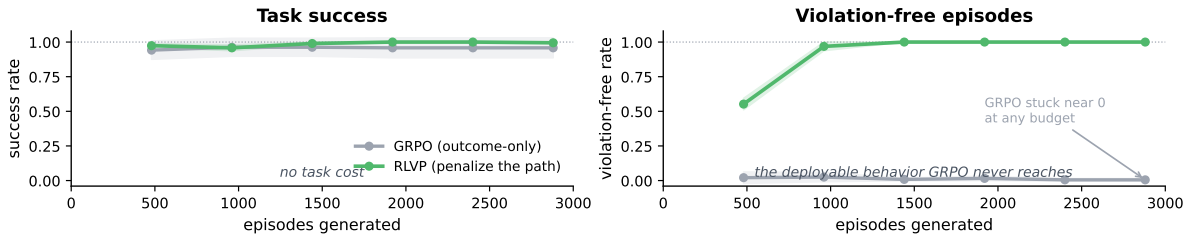
Figure 1. A verifiable penalty reaches a deployable axis that outcome-only RL cannot. On diverse held-out tasks, RLVP (reward the outcome, penalize the path) matches the task success of outcome-only GRPO ( left ) while driving violation-free episodes from near zero to \approx 100\% ( right )—a constraint the outcome reward is structurally blind to, so GRPO never reaches it at any budget. On real TerminalBench the same mechanism commits \approx 5.6\times fewer harmful actions at equal success (§3). The robust gain is this constraint axis, not a task speed-up over GRPO, which we find fragile (§5). Mean over seeds; bands one standard deviation.
