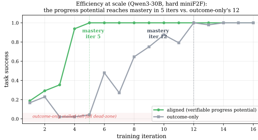
Figure 14. The speed gain holds at 30B on real theorems. On hard miniF2F with Qwen3-30B, the aligned potential reaches full success in five iterations while outcome-only takes twelve and stalls near zero early. Both saturate; the gain is speed, not final success.
