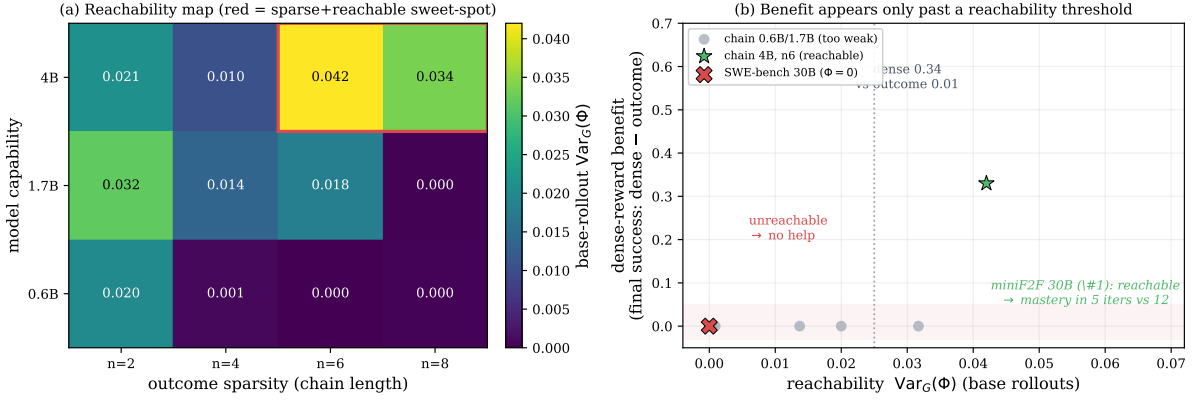
Figure 5. Reachability, measured cheaply, gates the dense-reward benefit. (a) \text{Var}_G(\Phi) on base-policy rollouts (no training) over model capability \times outcome sparsity: it rises with capability and peaks in the sparse-but-reachable corner (red). (b) The benefit of a dense reward (final-success gap, dense – outcome) against that same probe: zero where \text{Var}_G(\Phi) \approx 0 (the too-weak small models; the SWE null, \Phi=0 across 156 rollouts) and large where it is high (the 4B reachable chain; real theorem proving, #1, annotated). Benefit appears only past a reachability threshold. The controlled chain interior could not be filled (small-scale training is unreliable), so the positive evidence is the 4B point plus the real-domain anchors.
