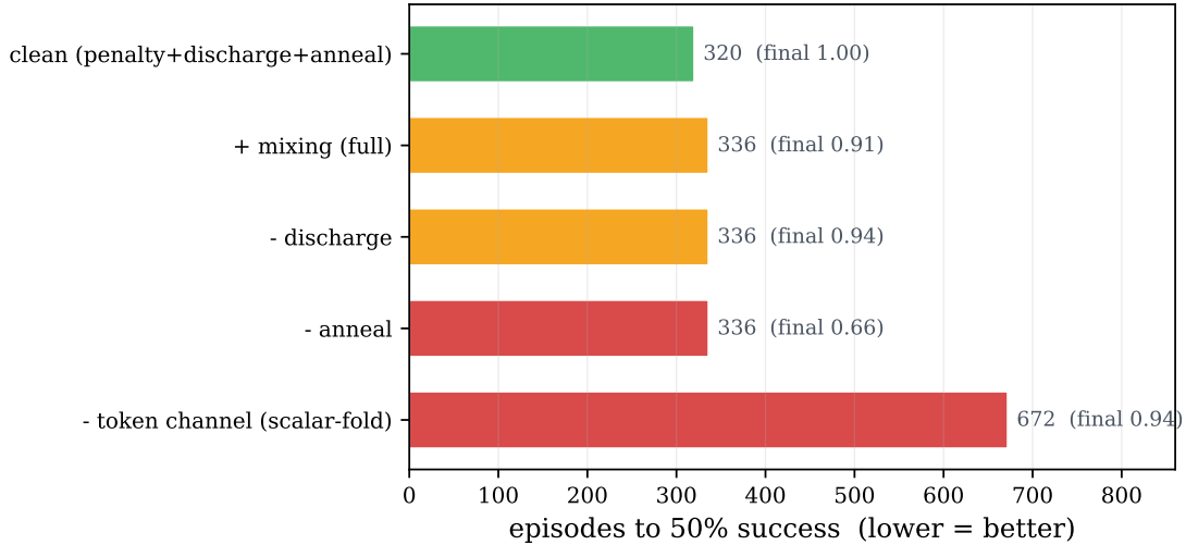
Figure 10. Component attribution on N=4 (episodes to threshold, final converged success annotated). The token-attached credit channel is the efficiency lever (folding into a scalar return doubles the cost). Annealing protects the ceiling, and the clean recipe is the best variant. A per-step length cost, helpful only on very long horizons, hurts here.
