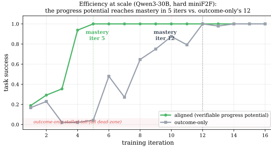
Figure 9. The efficiency gain holds at 30B on real theorems. On hard miniF2F with Qwen3-30B, the aligned verifiable-progress potential reaches full success in five iterations, while outcome-only takes twelve and stalls near zero for its first iterations (the all-fail dead-zone). Both saturate, so the gain is speed (more than twice as few iterations to mastery, and avoidance of the early dead phase), not a difference in final success.
