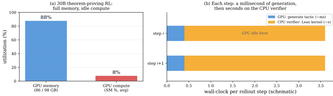
Figure 15. Verifiable agentic RL is often verifier-bound, not compute-bound. (a) During 30B theorem-proving RL the GPU runs at full memory but single-digit compute utilization. (b) Why: each rollout step spends a millisecond generating a tactic on the GPU, then seconds in the CPU-side Lean kernel verifying it, during which the GPU idles. Throughput then scales with verifier (environment) parallelism rather than accelerators. This holds for cheap CPU verifiers, though generation-heavy or learned-verifier workloads remain GPU-bound.
