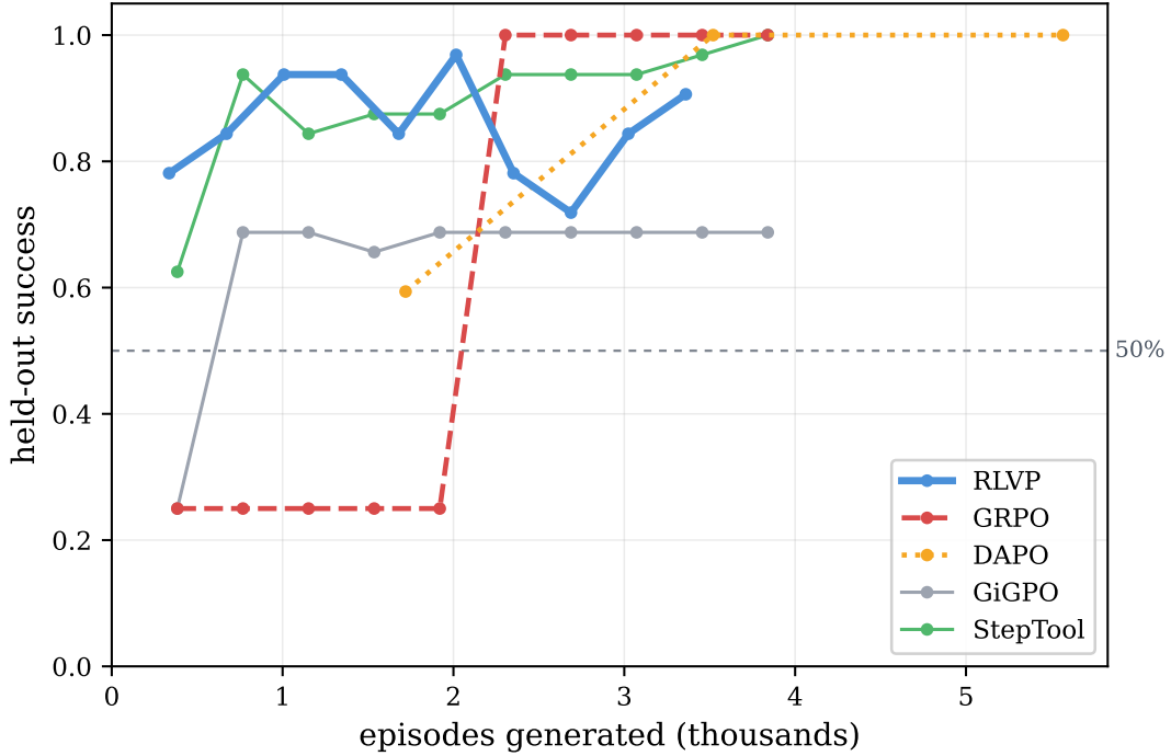
Figure 7. Sample efficiency on the calibrated hard task ( N=4 ): held-out success vs. episodes generated.
