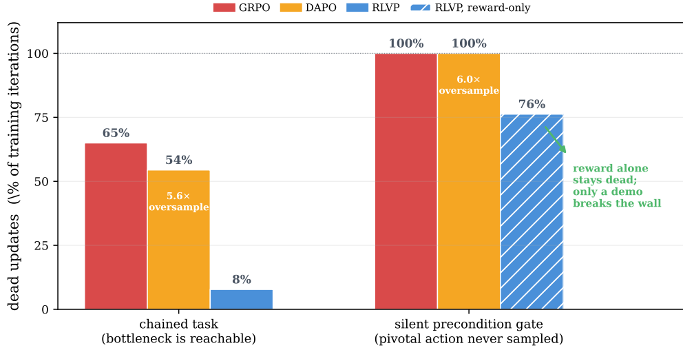
Figure 6. Dead updates across two regimes and three credit schemes. Fraction of training iterations whose update is dead, an all-fail group with zero reward spread (Qwen3-4B, 3-seed mean on the chained task). Chained task , where the bottleneck behaviour is reachable: outcome-only GRPO is dead 65% of the time, DAPO resamples away all-fail groups but still sits at 54% and pays a 5.6\times generation tax, and the admissible process reward (RLVP) cuts dead updates to 8%. Silent precondition gate (§9), where the pivotal action is never sampled: outcome and DAPO are dead on every iteration, and even reward-only RLVP (hatched) is dead 76% of the time, because no reward can credit a behaviour the policy never attempts, and only a demonstration seed breaks the wall. The cure for dead updates is not density but a reachable, admissible signal.
