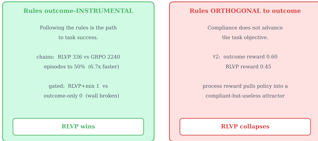
Figure 12. The boundary on a single axis: are the rules outcome-instrumental? When the verifiable rules are aligned with what success requires (chained and gated tasks: the workflow is the task), process rewards convert compliance into large outcome gains. When orthogonal to the reward ( \tau -bench with generic rules), the same machinery optimizes compliance into a degenerate policy.
