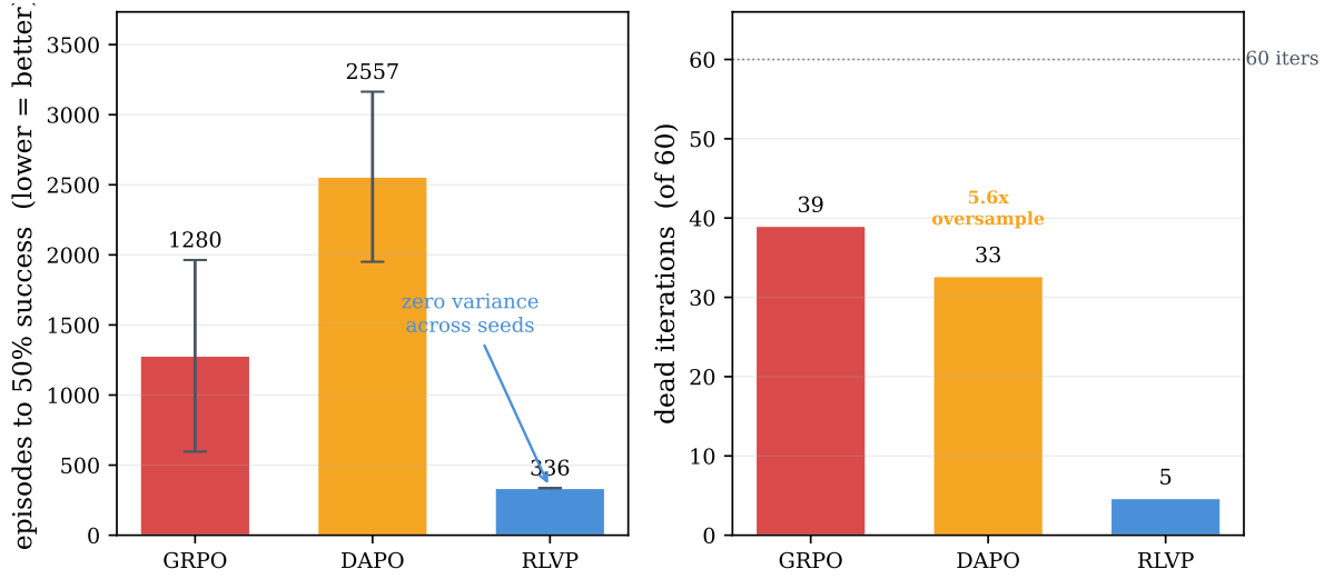
Figure 8. Headline efficiency comparison over three seeds. Left: episodes to the success threshold (lower is better). RLVP is several times faster than GRPO and DAPO and, unlike both, has near-zero seed variance. GRPO’s large error bar is the all-fail lottery. Right: the mechanism. GRPO and DAPO burn most iterations on dead or stalled updates, and DAPO additionally generates 5.6× the episodes it uses.
