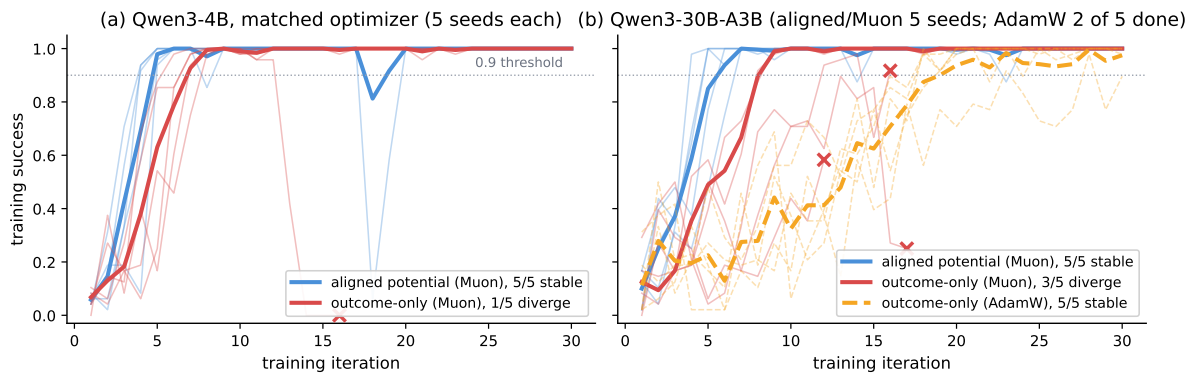
Figure 10. The aligned-potential recipe on real theorems (miniF2F algebra), five seeds per arm. Thin lines are seeds, thick lines the mean over stable seeds, \times marks a divergence-guard abort. (a) Controlled same-optimizer comparison at 4B: the aligned potential crosses the 0.9 threshold in 4.4 \pm 0.5 iterations vs. 7.0 \pm 0.7 for outcome-only—faster on every seed—and never diverges, while outcome-only loses one seed to entropy collapse. (b) At 30B, outcome-only faces a speed–reliability dilemma: under Muon it diverges on three of five seeds; under AdamW it is stable on all five seeds but takes \sim 3.6\times longer to master the task (threshold 19.2 \pm 1.9 vs. 5.4). The aligned potential is fast and stable on every seed at both scales.
