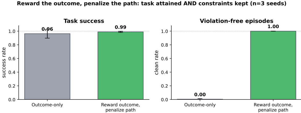
Figure 5. Reward-the-outcome-penalize-the-path attains the task and the constraints. Across diverse held-out tasks and model scales, outcome-only training solves the task but violates the outcome-neutral rules on nearly every episode (low “clean” rate). The two-channel recipe keeps task success high while driving violation-free episodes to near-100%, with small seed variance. Numbers are means over five seeds; error bars are one standard deviation.
