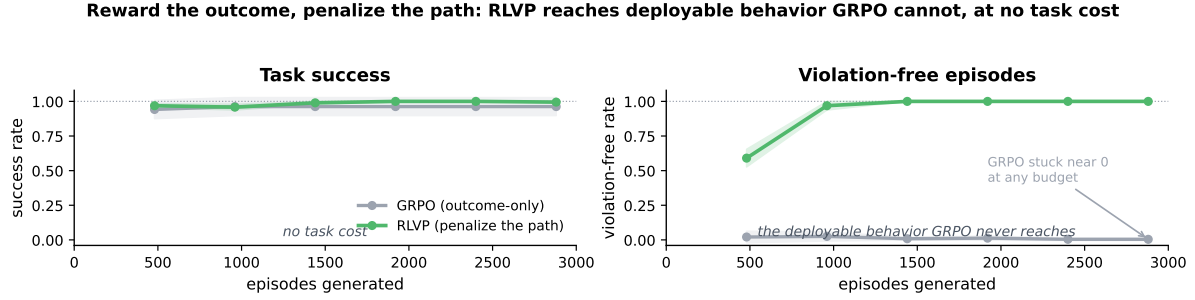
Figure 1. A verifiable penalty reaches a deployable axis outcome-only RL cannot. On diverse held-out tasks, RLVP (reward the outcome, penalize the path) matches the task success of outcome-only GRPO ( left ) while driving violation-free episodes from near zero to \approx 100\% ( right )—a constraint the outcome reward is blind to, so GRPO never reaches it at any budget. On TerminalBench the same mechanism commits \approx 5.6\times fewer harmful actions at equal success (§3); the sample-efficiency half (dense potentials) is treated in §5. Mean over seeds; bands \pm 1 s.d.
