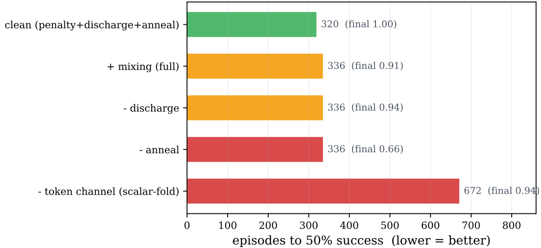
Figure 15. Component attribution for the potential on N=4 (episodes to threshold, converged success annotated). The token-attached credit channel is the efficiency lever (folding into a scalar return doubles the cost); annealing protects the ceiling; the clean recipe is best. A per-step length cost, useful only on very long horizons, hurts here.
