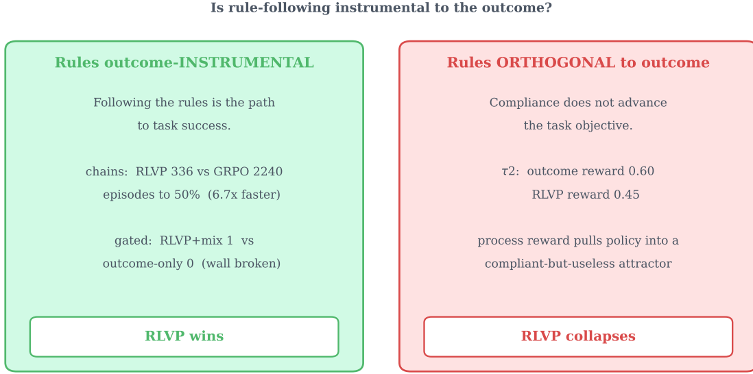
Figure 19. The boundary on one axis: are the rules outcome-instrumental? When the verifiable rules are aligned with what success requires (chained and gated tasks: the workflow is the task), the process channel converts compliance into large outcome gains. When orthogonal to the reward ( \tau -bench, generic rules), the same machinery optimizes compliance into a degenerate policy.
