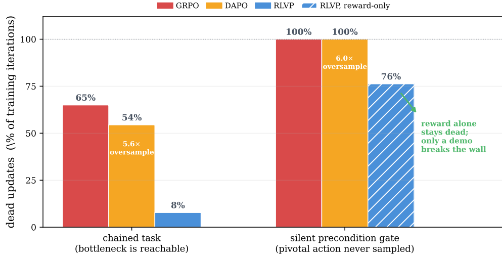
Figure 5. Dead updates across two regimes and three credit schemes. Fraction of training iterations whose update is dead—an all-fail group with zero reward spread (Qwen3-4B, 3-seed mean on the chained task). Chained task , where the bottleneck behaviour is reachable: outcome-only GRPO is dead 65% of the time; DAPO resamples away all-fail groups but still sits at 54% and pays a 5.6\times generation tax; the admissible process reward (RLVP) cuts dead updates to 8%. Silent precondition gate (§9), where the pivotal action is never sampled: outcome and DAPO are dead on every iteration, and even reward-only RLVP (hatched) is dead 76% of the time, because no reward can credit a behaviour the policy never attempts—only a demonstration seed breaks the wall. The cure for dead updates is not density but a reachable, admissible signal.
