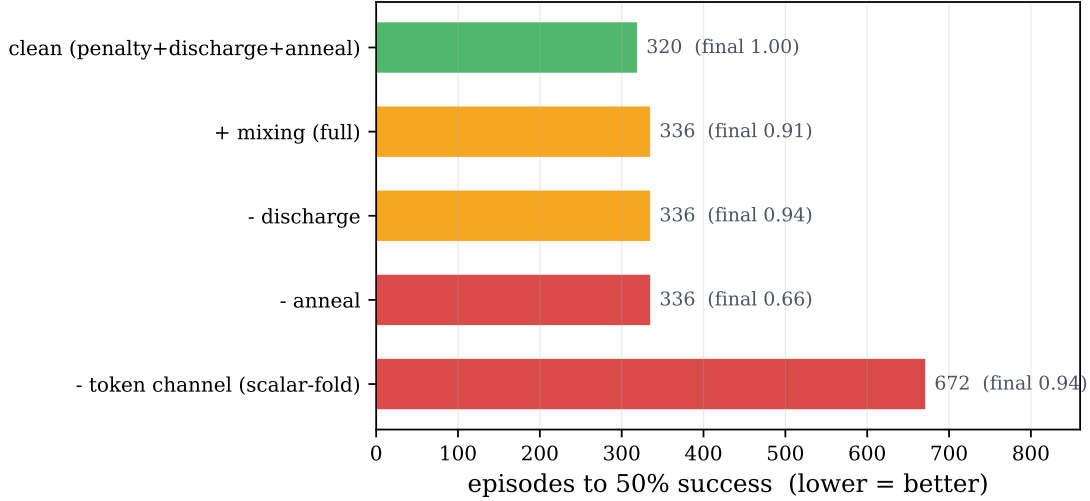
Figure 8. Component attribution on N=4 (episodes to threshold; final converged success annotated). The token-attached credit channel is the efficiency lever (folding into a scalar return doubles the cost); annealing protects the ceiling; the clean recipe is the best variant. A per-step length cost, helpful only on very long horizons, hurts here.
