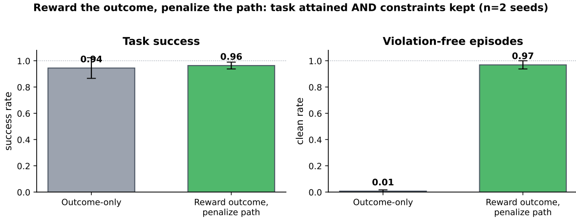
Figure 3. Reward-the-outcome-penalize-the-path attains the task and the constraints. Across diverse held-out tasks and model scales, outcome-only training solves the task but violates the outcome-neutral rules on nearly every episode (low “clean” rate). The two-channel recipe keeps task success high while driving violation-free episodes to near-100%, with small seed variance. Numbers are means over five seeds; error bars are one standard deviation.
