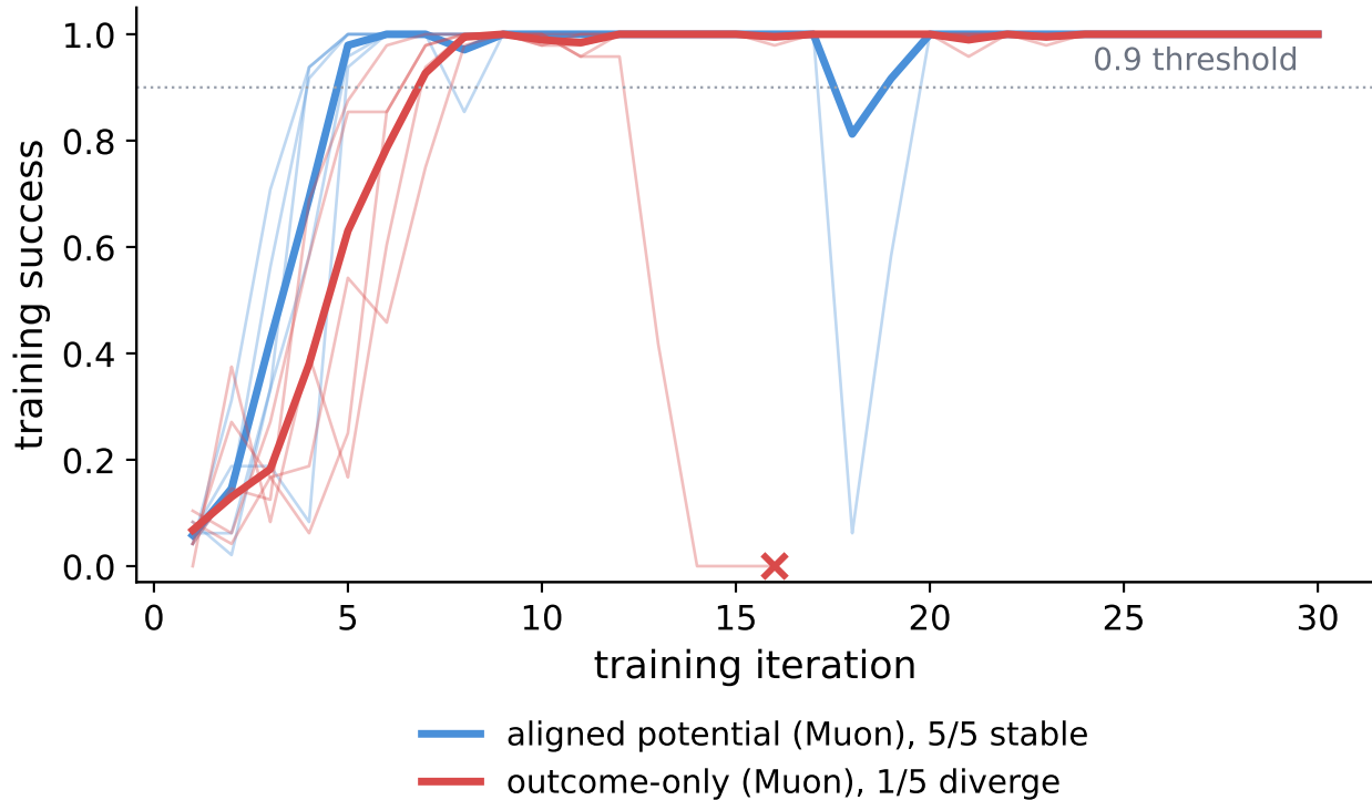
(a) Qwen3-4B, matched optimizer (5 seeds each)
