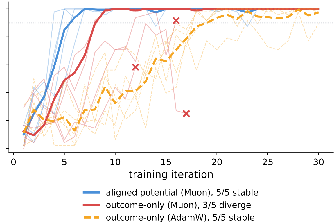
(b) Qwen3-30B-A3B (5 seeds per arm)
