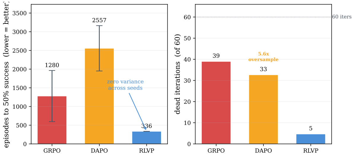
Figure 4. Headline comparison over three seeds. Left: episodes to reach 50% success (lower is better). RLVP is several times faster than GRPO and DAPO and—unlike both—has near-zero seed variance; GRPO’s enormous error bar reflects the all-fail-group lottery. Right: the mechanism behind the gap. GRPO and DAPO burn most iterations on dead or stalled updates, while DAPO additionally generates 5.6× more episodes than it uses. RLVP wastes almost no updates and no extra samples.
