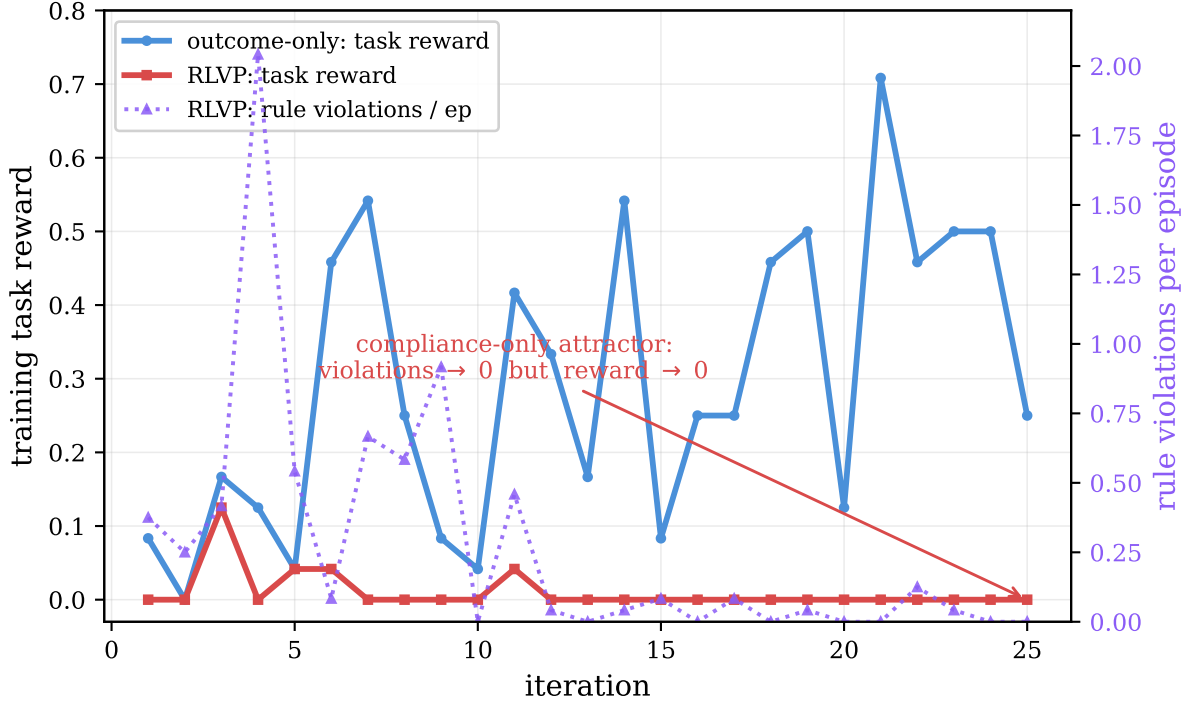
Figure 7. The compliance-only attractor on a real benchmark with orthogonal rules. Training on \tau -bench airline, outcome-only GRPO climbs in task reward while ignoring the structural rules. RLVP, whose generic structural rules are orthogonal to this benchmark’s reward, instead drives violations to zero by ceasing to attempt the risky task actions at all—its reward collapses to the floor. The process channel works perfectly; it just optimizes a quantity that does not move the outcome.
