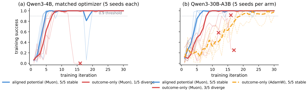
Figure 10. The aligned-potential recipe on real theorems (miniF2F algebra), five seeds per arm. Thin lines are seeds, thick lines the mean over stable seeds, \times marks a divergence-guard abort. (a) Controlled same-optimizer comparison at 4B: the aligned potential crosses the 0.9 threshold in 4.4 \pm 0.5 iterations vs. 7.0 \pm 0.7 for outcome-only—faster on every seed—and never diverges, while outcome-only loses one seed to entropy collapse. (b) At 30B, outcome-only faces a speed–reliability dilemma: under Muon it diverges on three of five seeds; under AdamW it is stable on all five seeds but takes \sim 3.6\times longer to master the task (threshold 19.2 \pm 1.9 vs. 5.4). The aligned potential is fast and stable on every seed at both scales.
