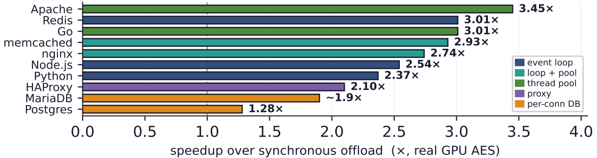
Figure 1. The headline result. Rerouting the offload through each server’s own concurrency recovers 1.3–3.5 \times across ten servers (real GPU AES, 1 MiB; up to 5.4 \times at 8 MiB; the databases pipeline a launch-bound op); zero-edit rerouting from outside the binary reaches 17.3 \times (§4). Color marks the concurrency model.
