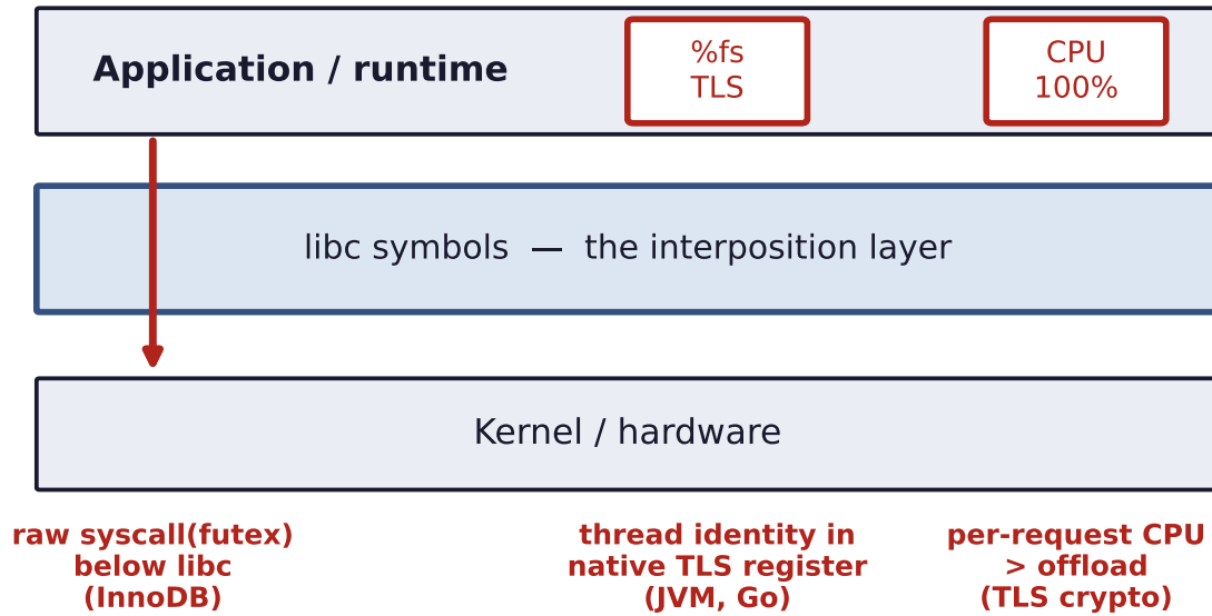
Figure 8. The interposition envelope. A preloaded library virtualizes the libc symbol layer, and reaches exactly the behavior that flows through it. Behavior escapes in three ways: below the layer (raw futex syscalls, InnoDB), beside it (thread identity in a native TLS register, the JVM and Go), and behind it (per-request CPU that already exceeds the offload).
