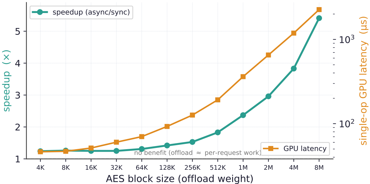
Overlap pays with offload weight (real GPU AES, single event loop)
