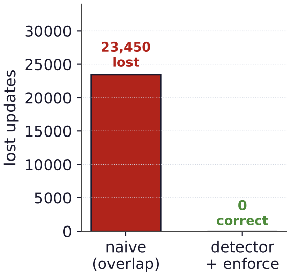
Shared-state safety (stock Redis)
