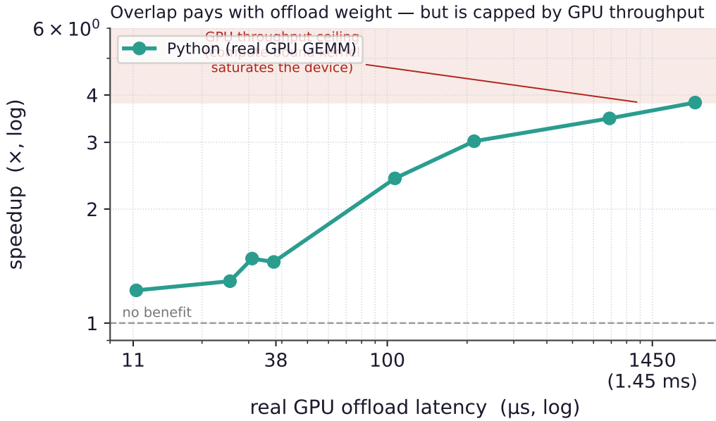
Figure 10. The predictive model, part two (measured, real GPU): overlap pays only when the offload outweighs per-request CPU work. Sweeping a real cuBLAS-GEMM offload from 11 \mu s to 1.45 ms on a single-event-loop server, the same edit gives no benefit for a light offload ( 1.2\times ) and rises to 3.8\times for a heavy one—capped there by the GPU’s throughput, as a compute-bound kernel saturates the device. This condition also explains the transparent runtime’s third wall.
