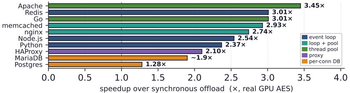
Figure 1. The headline result. Rerouting the offload through each server’s own concurrency recovers 1.3\text{--}3.5\times across ten servers (real GPU AES, 1 MiB; up to 5.4\times at 8 MiB; the databases pipeline a launch-bound op); zero-edit rerouting from outside the binary reaches 17.3\times (§4). Color marks the concurrency model.
