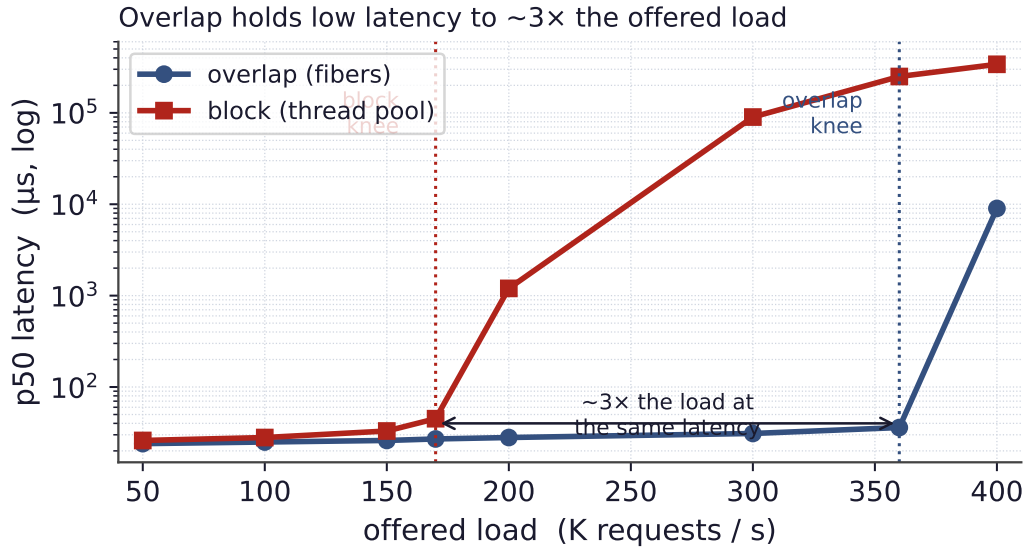
Figure 12. Latency under load. With an open-loop arrival process, blocking on the offload drives the median latency up at its saturation point, while overlapping holds low latency to roughly 3\times the offered load before its own knee. Overlap is a latency win, not only a throughput win.
