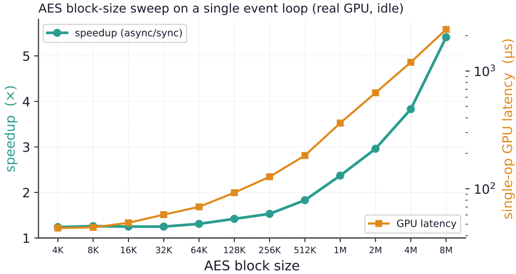
Figure 14. The same data: real-GPU AES speedup (left axis) and measured single-op GPU latency (right axis) versus AES block size, consecutive powers of two from 4 KiB to 8 MiB.
