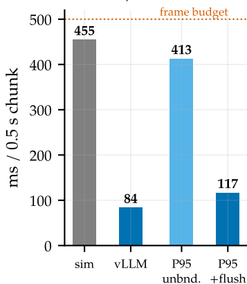
(b) 5.4 \times faster than the simulator; flush bounds P95
