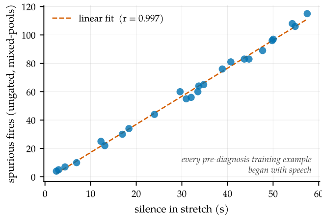
Figure 8. Silence incompetence. Spurious fires of the ungated mixed-pools model track the silence content of each stretch almost perfectly; ungated recall is therefore uninterpretable, and all reported arms run behind the energy gate.
