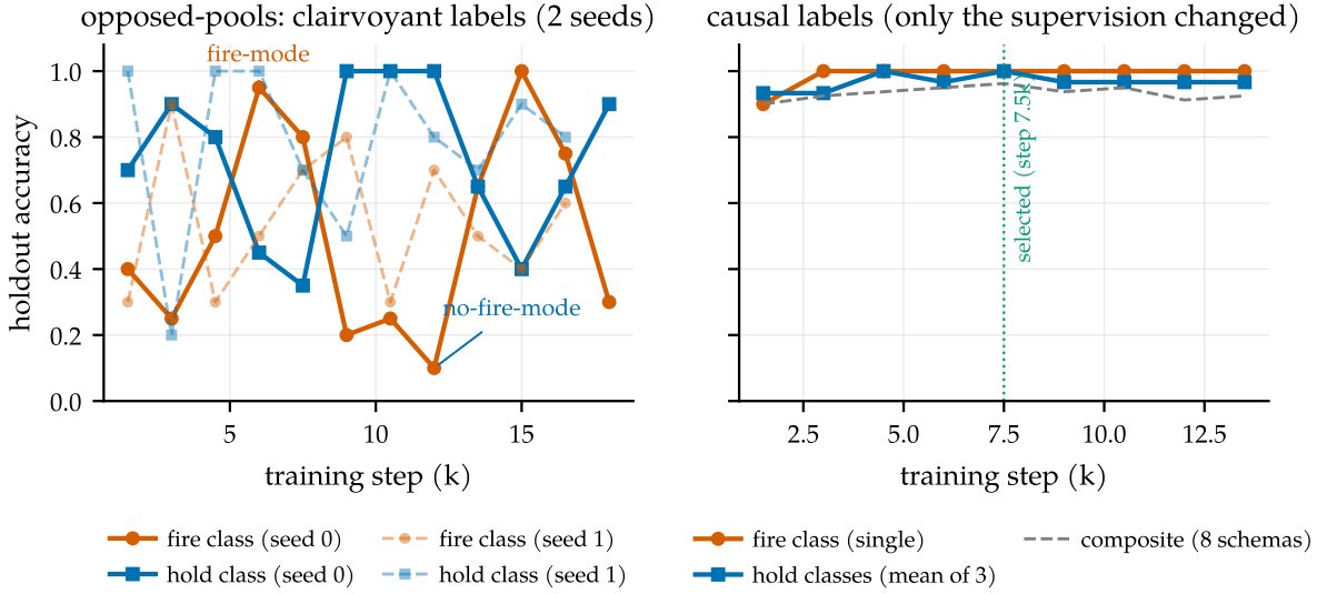
Figure 5. The fingerprint of contradictory supervision. Left: under the opposed-pools composition, holdout accuracy oscillates for the entire run between a fire-mode and a no-fire-mode attractor, reproducibly across two training seeds (solid, dashed); the oscillation is a property of the labels, not a seed. Right: the causal recipe of §3.2, with the same architecture, adapter, and data volume and only the labels changed, climbs monotonically, with both classes at ceiling simultaneously from step 3k on.
