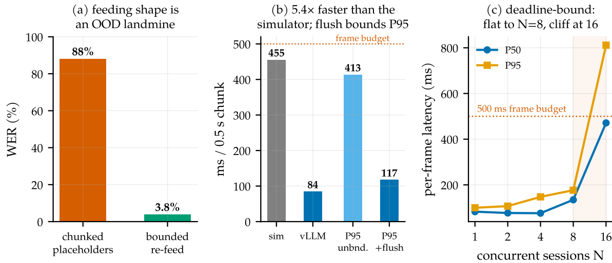
Figure 13. Serving on real infrastructure. (a) Feeding shape: per-chunk placeholders are out-of-distribution; bounded re-feed is correct. (b) Per-chunk compute on vLLM vs. the transformers simulator; the force-flush bounds the P95 tail. (c) Concurrent sessions per engine on a 0.15-GPU slice: flat to N=8 , cliff at 16.
