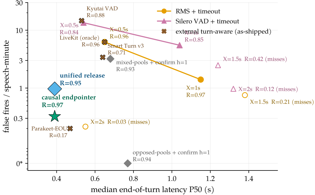
Figure 2. The causal model escapes the timeout curve. Median end-of-turn latency vs. false fires (log scale; 0* plotted at 0.05) on identical audio, detector, and scoring (§4.1). A silence timeout can only slide along its curve; the causally supervised model sits strictly inside the whole family because it reads completeness, firing 0.39 s after a finished thought while holding through a 1.4 s mid-sentence pause.
