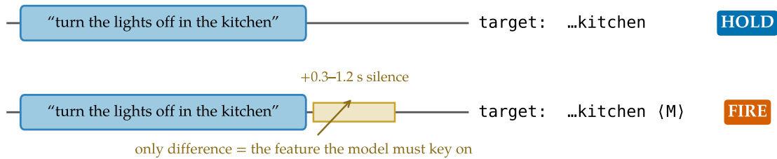
Figure 10. The minimal-pair device. Each complete utterance appears twice: without a silence tail (target: transcript only) and with a 0.3–1.2 s tail (target: transcript + marker). The only difference between the opposite-labeled examples is the observable the model must key on.
