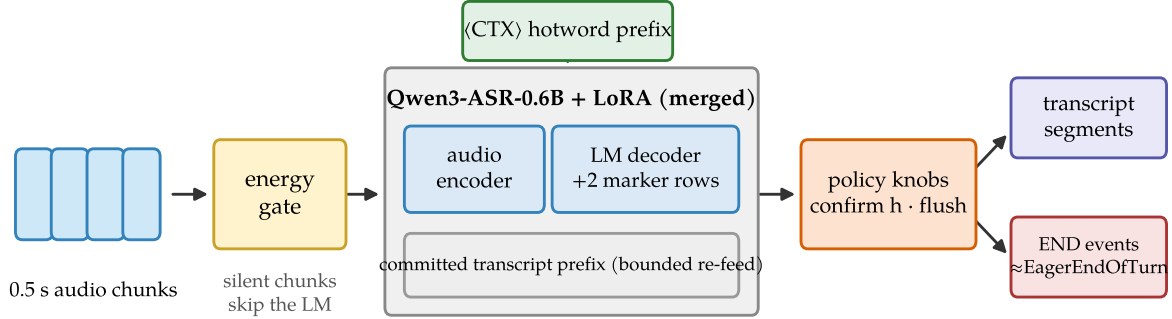
Figure 3. System shape. Audio chunks pass an energy gate; the merged LoRA model transcribes the current bounded segment with the <CTX> prefix in the system slot and may emit marker tokens; two policy knobs sit behind the model. Outputs are transcript segments plus END events, the same event shape as Flux’s EagerEndOfTurn .
