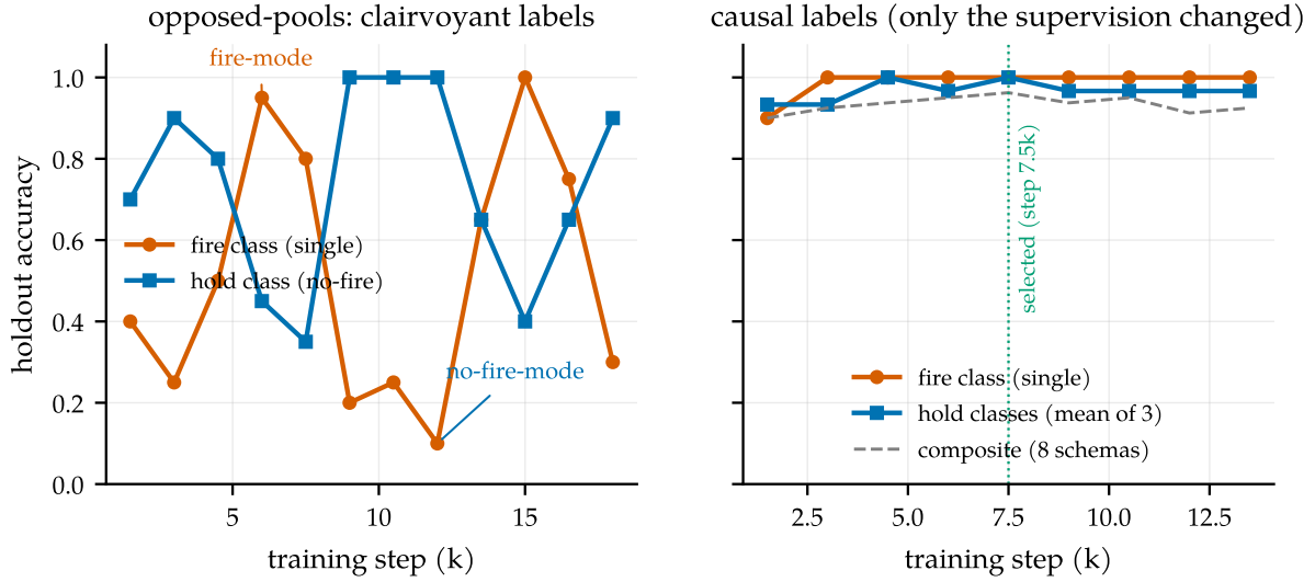
Figure 5. The fingerprint of contradictory supervision. Left: under the opposed-pools recipe (clairvoyant labels), holdout accuracy oscillates for the entire run between a fire-mode attractor (fire class \approx 1.0 , hold class \approx 0.4 ) and a no-fire-mode attractor (fire \approx 0.1 , hold \approx 1.0 ): the pools assign opposite targets to causally identical audio, so no single policy satisfies both. Right: the causal recipe of §4 — same architecture, same LoRA recipe, same data volume, only the labels changed — climbs monotonically, and both classes sit at ceiling simultaneously from step 3k on.
