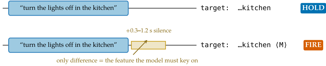
Figure 4. The minimal-pair device. Each complete utterance appears twice in the training data: without a silence tail (target: transcript only) and with a 0.3–1.2 s tail (target: transcript + marker). The only difference between the opposite-labeled examples is the observable the model must key on. This construction is what removes the training pathology of Figure 5.
