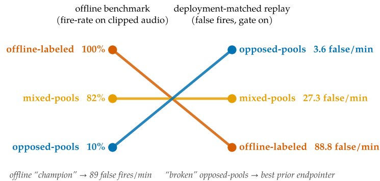
Figure 8. The ranking inversion. Left: the legacy offline benchmark (fire-rate on clips cut at end-of-speech). Right: the deployment-matched replay benchmark (false fires per speech-minute, energy gate on; full metrics in Table 5). The offline champion fires 89 times per speech-minute mid-utterance — its offline strength is a premature-fire pathology once audio keeps flowing. The opposed-pools model, written off at 10% offline, is the best prior endpointer. Both historical ship decisions were wrong.
