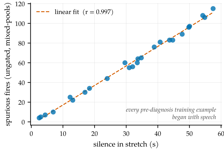
Figure 7. Silence incompetence. Spurious fires of the ungated mixed-pools model against the silence content of each benchmark stretch: the model hallucinates text and sprays markers on silence at \sim 1.9 fires/s ( r = 0.997 ), because every pre-diagnosis training example begins with speech while a real channel is mostly silence (13 of 22 minutes here). Consequence: ungated recall is uninterpretable — a random 1.9 Hz spammer scores 0.96 recall against the tolerance window. The fix costs one line (RMS energy gate), and the causal recipe additionally bakes silence schemas into training (Table 2, #7–8).
