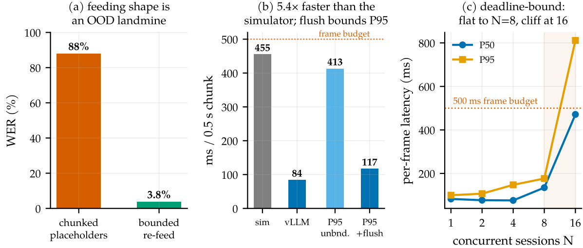
Figure 10. Serving on real infrastructure. (a) Feeding shape: per-chunk audio placeholders are out-of-distribution for a model trained on single segments (88% WER); bounded re-feed of the last window costs a re-encode but is correct (3.8%). (b) Per-chunk compute: the vLLM path is 5.4\times faster than the transformers simulator used for all pre-serving latency numbers; the max-segment force-flush also bounds the P95 tail. (c) Concurrent sessions per engine on a 0.15-GPU slice: flat to N=8 , cliff at 16 — the deadline binds, not memory.
