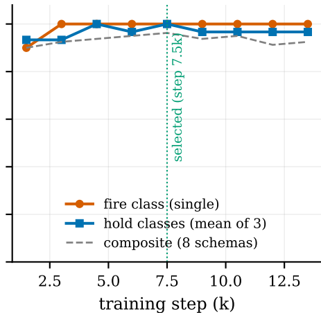
v9: causal labels (only the data changed)
