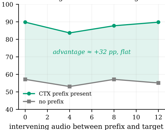
biasing survives session length
