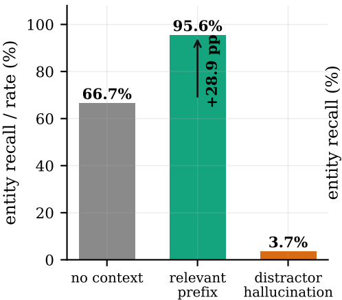
Earnings-22 hotword biasing
