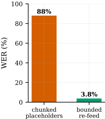
(a) feeding shape is an OOD landmine
