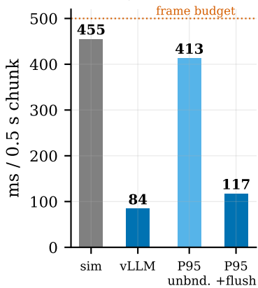
(b) 5.4\times faster than the simulator; flush bounds P95
