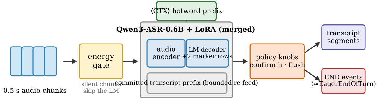
Figure 2: System shape. Audio chunks pass an RMS energy gate (silent chunks never start a segment, so mostly-silent sessions are nearly free); the merged LoRA model transcribes the current bounded segment with the <CTX> hotword prefix in the system slot and may emit marker tokens; two policy knobs (confirm horizon, max-segment force-flush) sit behind the model. Outputs are transcript segments plus END events — the same event shape as Flux’s EagerEndOfTurn .
