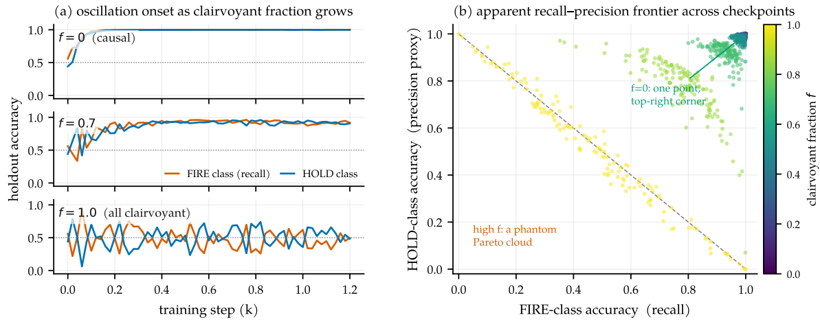
Figure 12. The mechanism, isolated. A \sim 30\text{k} -parameter transformer on a synthetic stream with a tunable clairvoyant-label fraction f . (a) Holdout trajectories: monotone convergence at f=0 , visible noise at f=0.7 , bistable mode-oscillation at f=1.0 . (b) Every checkpoint’s (fire recall, hold precision), colored by f : the causal run collapses to one top-right point; high f spreads checkpoints into an anti-diagonal cloud, a phantom Pareto frontier traced by one oscillating model.
