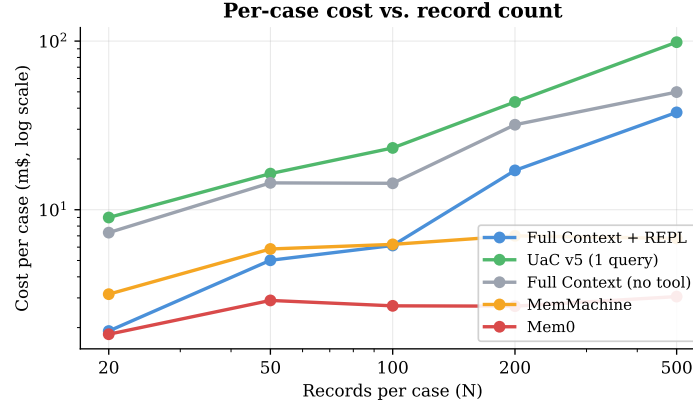
Figure 6. Per-case Gemini 3 Flash cost vs. record count N (log-log). UaC v5 and Full Context costs grow with N (more records to structure or read in-head); FC+REPL grows fastest because the records JSON is re-included in the LLM’s context every tool turn. Retrieval-based systems (MemMachine, Mem0) are cheap but bottom out on accuracy (Figure 5).
