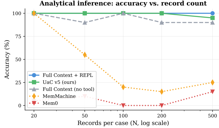
Figure 5. Analytical inference: accuracy vs. record count N (log scale). Code-executable representations (UaC v5, FC+REPL) stay at or above 95% across the full range. Full Context degrades past N=100 (90% at N=200 and N=500 ) as the LLM miscounts. MemMachine collapses from 100% to 15–25% as more records become relevant than top- k retrieval can return. Mem0 remains near zero throughout.
