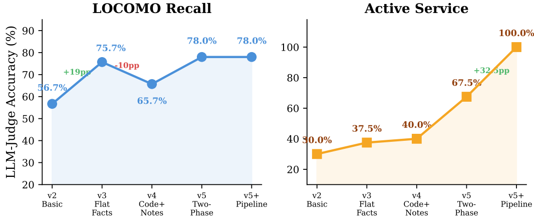
Figure 8. Ablation study showing the impact of each architectural decision (5-conv Locomo, n=300 ). Left: Locomo recall improves +19pp with append-only extraction ( v2 \rightarrow v3 ), drops -10pp with incremental code overwrite ( v3 \rightarrow v4 ), recovers and exceeds with two-phase separation ( v5 ). Right: Active Service improves steadily with code structure, with the constraint pipeline adding +32.5pp ( v5 \rightarrow v5+\text{pipeline} ).
