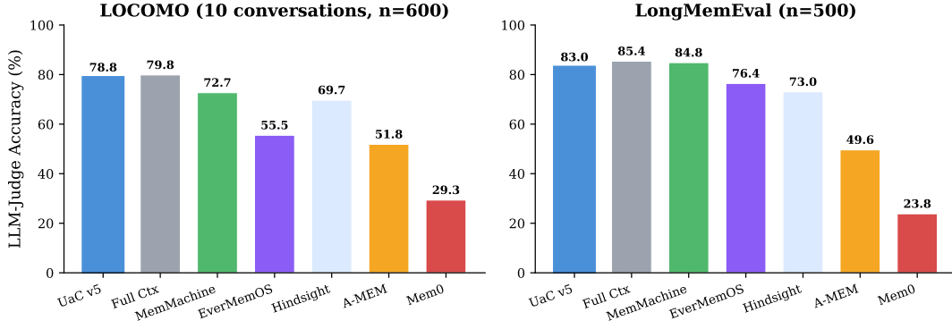
Figure 4. Standard benchmark comparison. All six memory systems share the same evaluation data: the full 10-conversation LOCOMO benchmark (600 QAs) and the full 500-question LongMemEval benchmark. Full Context is the upper bound (all raw text passed to the LLM).
