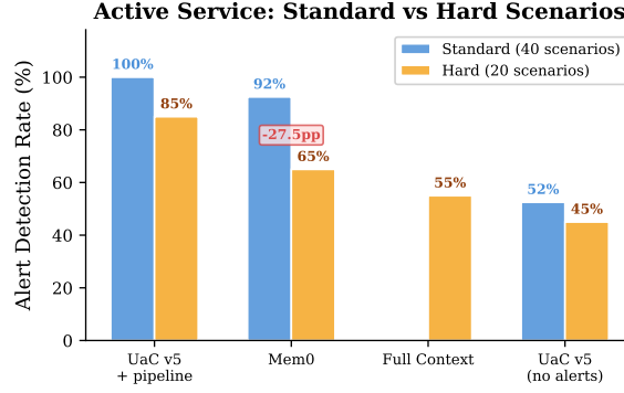
Figure 7. Active Service: standard vs. hard scenarios. On hard arithmetic (multi-step dates, compound constraints, tax calculations), live Mem0 drops 10pp (90.0%→80.0%), simulated Mem0 drops 27.5pp (92.5%→65.0%), and live A-MEM drops to 30.0%; UaC v5 drops only 15pp (100%→85.0%).
