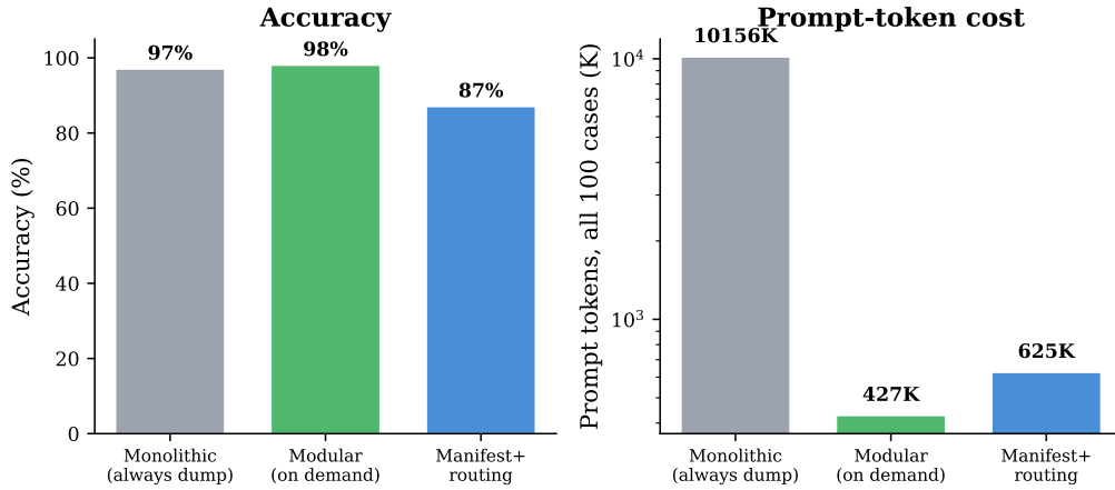
Figure 9. Modularity / Progressive Disclosure ablation (100 cases, 500 records). Left: modular loading matches or beats the monolithic upper bound; the manifest variant trails by 10pp due to mis-routing. Right: prompt-token cost drops 24 \times when only the relevant domain is loaded.
