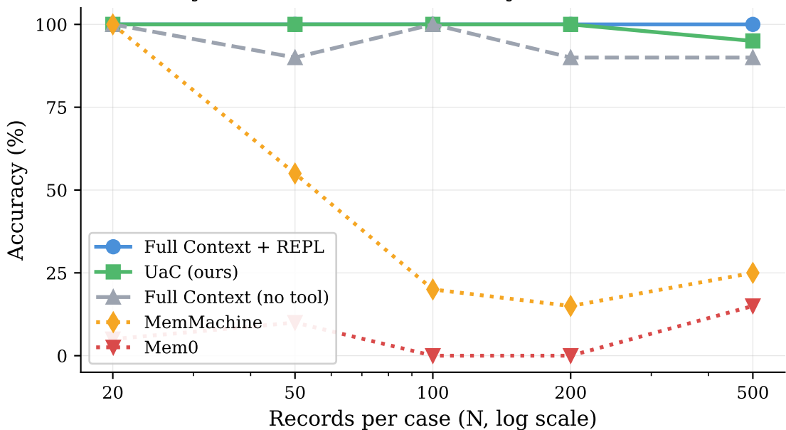
Analytical inference: accuracy vs. record count
