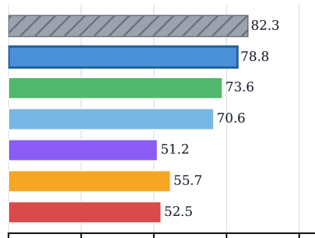
Judge accuracy
