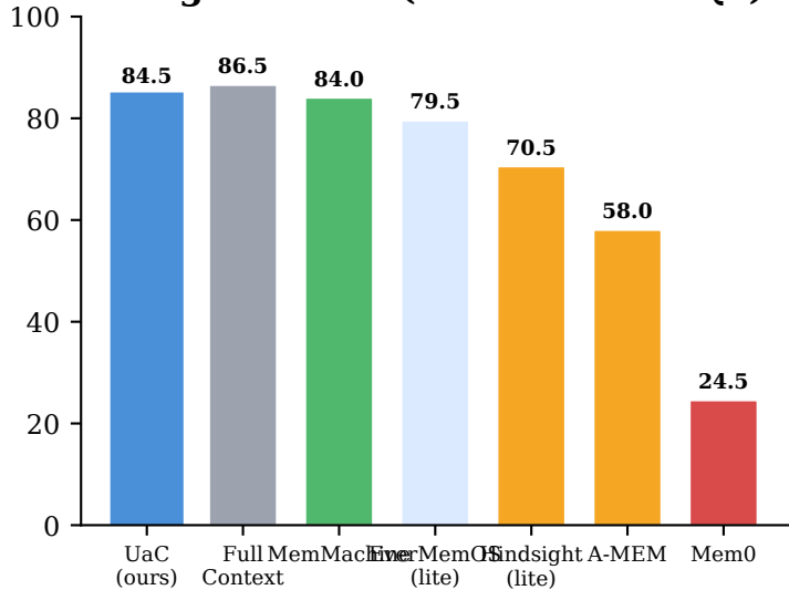
LongMemEval (200 stratified Qs)
