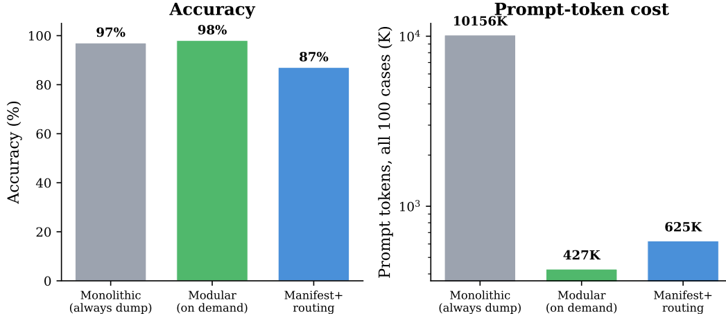
Figure 9: Modularity / Progressive Disclosure ablation (100 cases, 500 records). Left: modular loading matches or beats the monolithic upper bound; the manifest variant trails by 10pp due to mis-routing. Right: prompt-token cost drops 24× when only the relevant domain is loaded.
