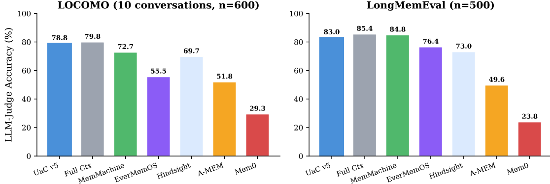
Figure 4: Standard benchmark comparison. All six memory systems share the same evaluation data: the full 10-conversation Locomo benchmark (600 QAs) and the full 500-question LongMemEval benchmark. Full Context is the upper bound (all raw text passed to the LLM).
