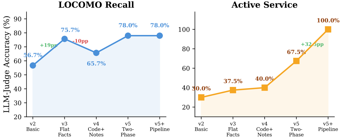
Figure 8: Ablation study showing the impact of each architectural decision (5-conv LOCOMO, n=300 ). Left: LOCOMO recall improves +19pp with append-only extraction (v2→v3), drops -10pp with incremental code overwrite (v3→v4), recovers and exceeds with two-phase separation (v5). Right: Active Service improves steadily with code structure, with the constraint pipeline adding +32.5pp (v5→v5+pipeline).
