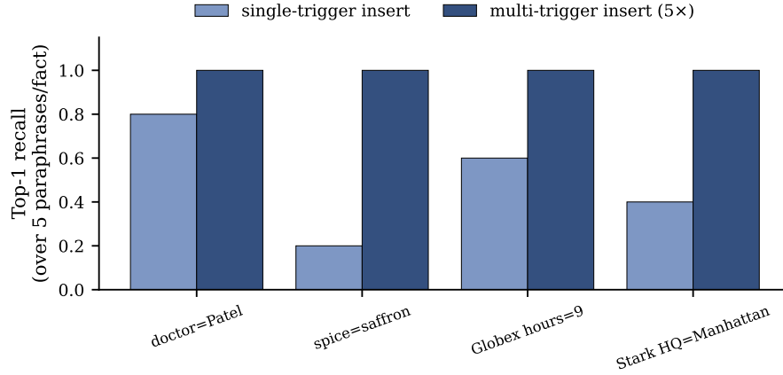
Figure 20. Paraphrase generalisation across 4 facts \times 5 paraphrases each. Single-trigger insertion gets 50% top-1 for free (suffix N-gram overlap); multi-trigger insertion (insert at all 5 paraphrases) gets 100% at 5 \times the per-fact OPT cost.
