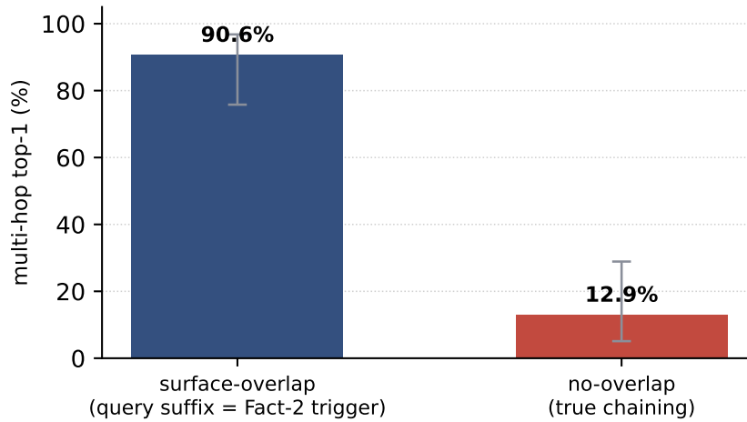
Figure 10. Multi-hop reasoning over Engram-inserted facts ( n=63 chained pairs on Mini-Engram-d20, two OPT-15 insertions per item). Per-fact direct recall is 99.2% (both facts are insertable), so the gap is chaining, not insertion. When the query’s suffix N-gram coincides with Fact-2’s trigger, the gate fires and recall is 90.6%; when true chaining is required, it collapses to 12.9% (Wilson 95% CIs shown). The gate is a surface-N-gram hash—it matches, it does not compose.
