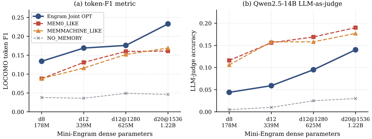
Figure 9. LOCOMO single-hop, full 10 conversations, scaling with Mini-Engram dense size. (a) Token-F1: User-as-Engram Joint OPT (blue) beats every retrieval baseline at every scale. (b) LLM-judge accuracy (Qwen2.5-14B-Instruct): the ranking flips—retrieval baselines (MEM0_LIKE, MEMMACHINE) beat Joint OPT by 0.05–0.10 because token-F1 over-credits Engram for the correct first answer token despite a noisy continuation.
