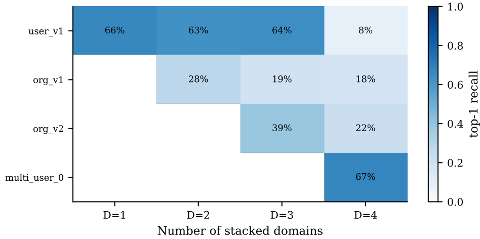
Figure 21. Multi-domain additive composition heatmap. Each cell shows per-domain top-1 recall when D domains are stacked. Heavy degradation when domains share trigger templates (high address overlap). Disjoint-template domains (corp + user, demonstrated in main text) compose without loss.
