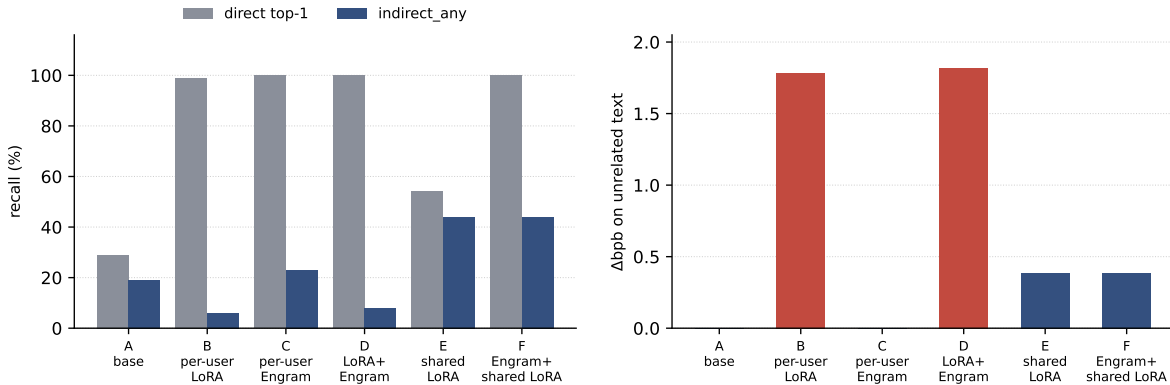
Figure 12. The six parametric conditions on n=20 test users (Mini-Engram-d20, seed S0). Left: F (Engram + shared LoRA) matches per-user LoRA’s direct recall (100% vs. 99%) while delivering 7.4\times its indirect_any (44% vs. 6%); neither the per-user Engram (C, no skill) nor the shared LoRA alone (E, never saw the user’s facts) suffices. Right: F adds zero contamination on top of the shared skill ( \Delta\text{bpb} +0.386 = \text{E} ), while per-user LoRA (B) and the naive LoRA+Engram stack (D) pay +1.78/+1.82 . RAG conditions (G–J) appear in Figure 24; 3 seeds in Appendix O (3-seed mean F 41%, B 7%).
