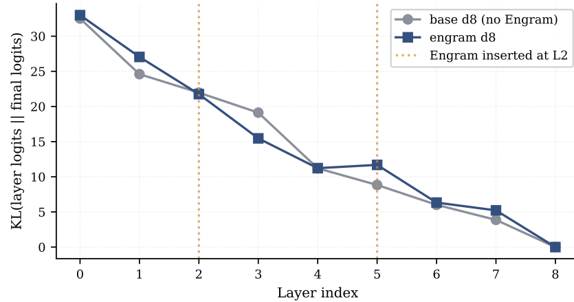
Figure 17. LogitLens KL by layer (Mini-Engram-d8 vs. base-d8). Engram converges faster at layer 3 (–3.66 KL gap), confirming Cheng et al.’s effective-deepening claim at our scale (stage 4 of the mechanism above).
