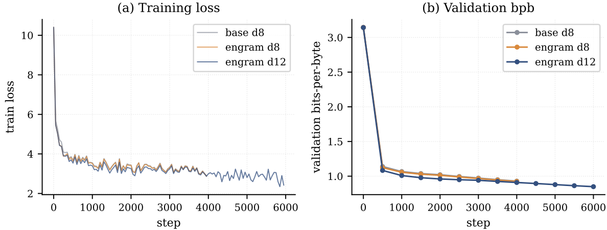
Figure 18. Mini-Engram pretraining curves. Engram d8 reaches lower validation bpb than base d8 at iso-FLOPs (matching the paper’s finding at much smaller scale); engram d12 is substantially better thanks to the larger backbone and longer training.
