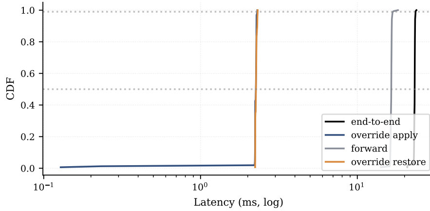
Figure 22. Per-request latency CDF on Mini-Engram-d12 (30 users \times 50 facts \times 600 requests). Override apply (blue) and restore (orange) are both sub-3 ms at p99; the forward pass (grey) dominates total latency (black).
