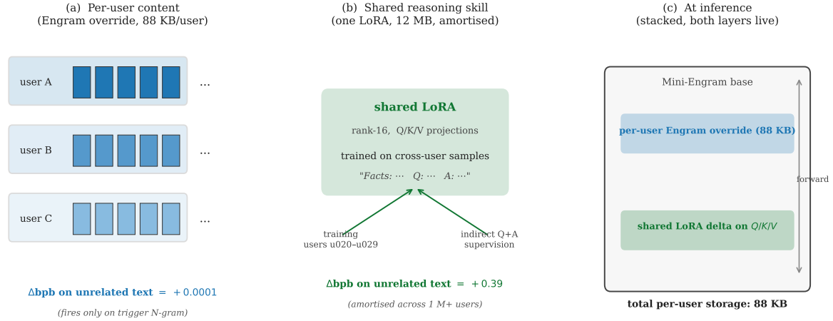
Figure 11. The layered architecture splits personal memory by who owns it and how often it changes. (a) Per-user content is a small Engram-row override (88 KB/user) that fires only on its trigger N-gram, so it perturbs unrelated text by \Delta\text{bpb} = +0.0001 . (b) The shared reasoning skill is a single rank-16 LoRA trained on cross-user indirect-QA samples; its \Delta\text{bpb} = +0.39 contamination is paid once and amortised across all users. (c) At inference both layers are live on the frozen Mini-Engram base.
