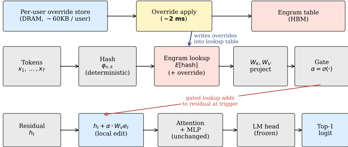
Figure 8. EngramServer architecture. Per user, an override map of (row index, row vector) pairs lives in DRAM. On each request, the server saves the originals at the affected addresses ( \sim 2 ms), writes the user’s overrides, runs the forward pass, then restores. The Engram lookup at the configured layer transparently sees the override values; the gate fires only at the trigger N-gram. There is no router and no graph rewrite.
