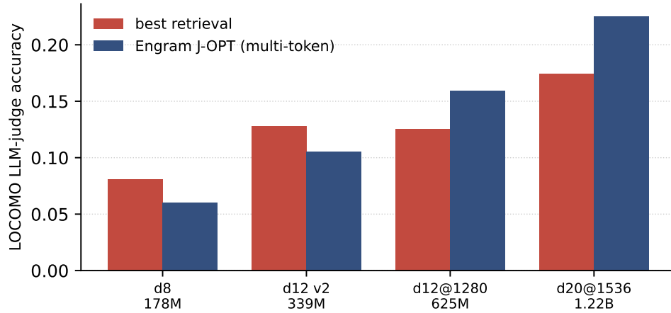
Figure 16. LOCOMO single-hop under an LLM judge (Qwen2.5-14B), matched multi-token pipeline. First-token OPT lets token-F1 over-credit Engram for a correct first token over a noisy continuation (Figure 15); training the full answer with multi-token Joint-OPT fixes this and overtakes the best retrieval baseline from d12@1280 upward (+27% at 625 M, +29% at 1.22 B). Below that cross-over the dense backbone is too small for the continuation to fall into place after the Engram-anchored prefix.
