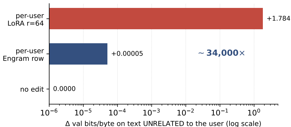
Figure 2. Architectural contamination on held-out text, Mini-Engram-d20 (canonical seed S0, n=20 users). A per-user LoRA more than triples val bpb on text unrelated to the user’s facts (+1.784; per-user range [+0.44, +3.74] ; 17/20 users worse), while a per-user Engram row leaves it unchanged to four decimals (+0.00005; 0/20 worse)— \sim 34,000\times less, by design. The 3-seed mean ratio is \sim 33,000\times (Appendix O).
