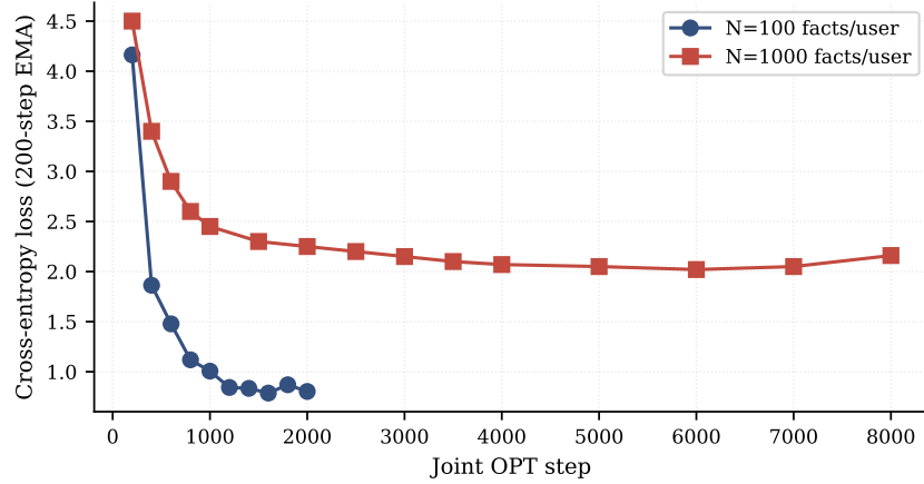
Figure 25. Joint OPT convergence on Mini-Engram-d12. At 100 facts/user, loss converges to 0.8 within 1500 steps; at 1000 facts, loss saturates around 2.0 due to higher within-user fact-density interference (Section 5.2).
