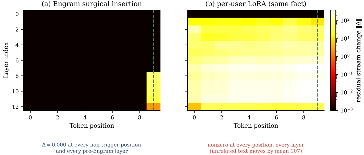
Figure 6. Addressed write vs. global function-bend. Per-layer, per-position residual-stream change \|x_{\text{after}}^{(\ell)} - x_{\text{before}}^{(\ell)}\| on the same trigger sentence and base (Mini-Engram-d12@1280, log colour scale). (a) An Engram row insertion is exactly 0.000 at every position before the Engram layer (causality) and at every non-trigger position after it—only the trigger column moves. (b) A per-user LoRA fit to the same single fact moves the residual at every position and every layer, and perturbs unrelated text (“The capital of France is”) by mean 107. Storing a fact in a shared function changes the function everywhere; storing it at an address does not.
