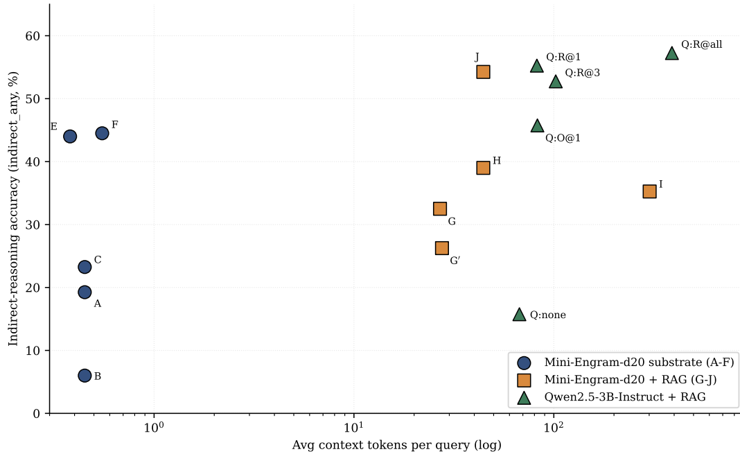
Figure 24. Indirect-reasoning accuracy ( indirect_any ) vs. avg context tokens per query on the 20-user split. F (layered) and E (shared LoRA only) anchor the 0-context end; J (RAG top-3 + shared LoRA) lifts accuracy to 54% at 44 context tokens; Qwen-3B + RAG reaches 55–57% at 82–390 tokens on a \sim 2\times larger backbone. Naive RAG on the same Mini-Engram-d20 base (G/H/I) sits below F: putting facts in context is not the same as having the reasoning skill.
