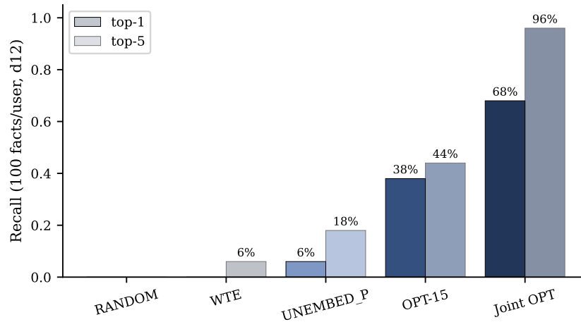
Figure 19. Top-1 and top-5 recall at 100 facts/user, Mini-Engram-d12. RANDOM (control) confirms our signal isn’t noise; UNEMBED_P alone is too weak; OPT-15 helps; Joint OPT closes most of the gap to full LoRA fine-tuning at 161\times less storage.
