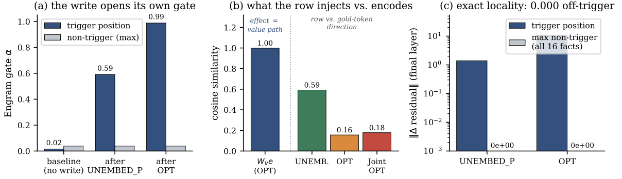
Figure 7. The mechanism on the trained model (Mini-Engram-d20, 16 facts). (a) The write opens its own gate: the trigger-position gate \alpha rises from 0.02 to 0.99 (OPT) while non-trigger positions stay at 0.04. (b) The deployed row’s residual change is cosine 0.999 to its value-path projection W_{ve} (left bar); what the row encodes relative to the gold token’s unembedding is exact for the closed-form solution (0.59) and drifts as gradient OPT/Joint-OPT trade direct gold-alignment for higher recall (0.16–0.18). (c) Exact locality: the maximum non-trigger residual change over all 16 facts is 0.000 for both strategies, versus an order-1 change at the trigger.
