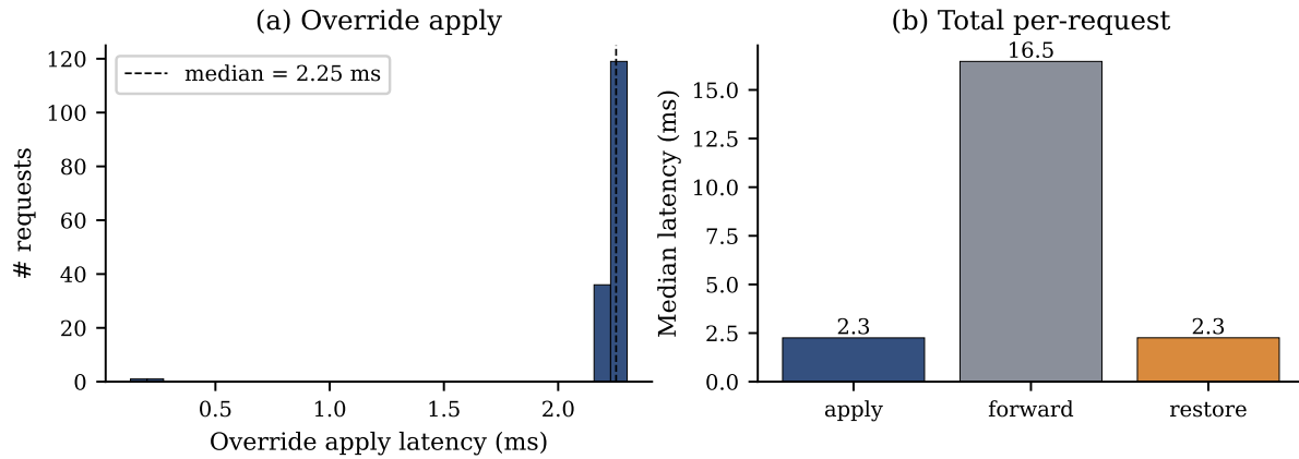
Figure 23. Per-request latency breakdown, Mini-Engram-d12 (30 users \times 50 facts \times 600 requests). (a) Override-apply latency: median 2.2 ms. (b) Median per-request latency by component: apply (2.3 ms) + forward (16.5 ms) + restore (2.3 ms); the frozen forward pass dominates, and the override apply+restore overhead ( \sim 4.6 ms) is under 20% of the 23.2 ms end-to-end median.
