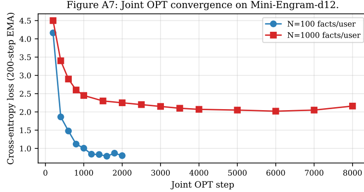
Figure 13: Joint OPT convergence on Mini-Engram-d12. At 100 facts/user, loss converges to 0.8 within 1500 steps; at 1000 facts, loss saturates around 2.0 due to higher within-user fact-density interference (Section 6.2).
