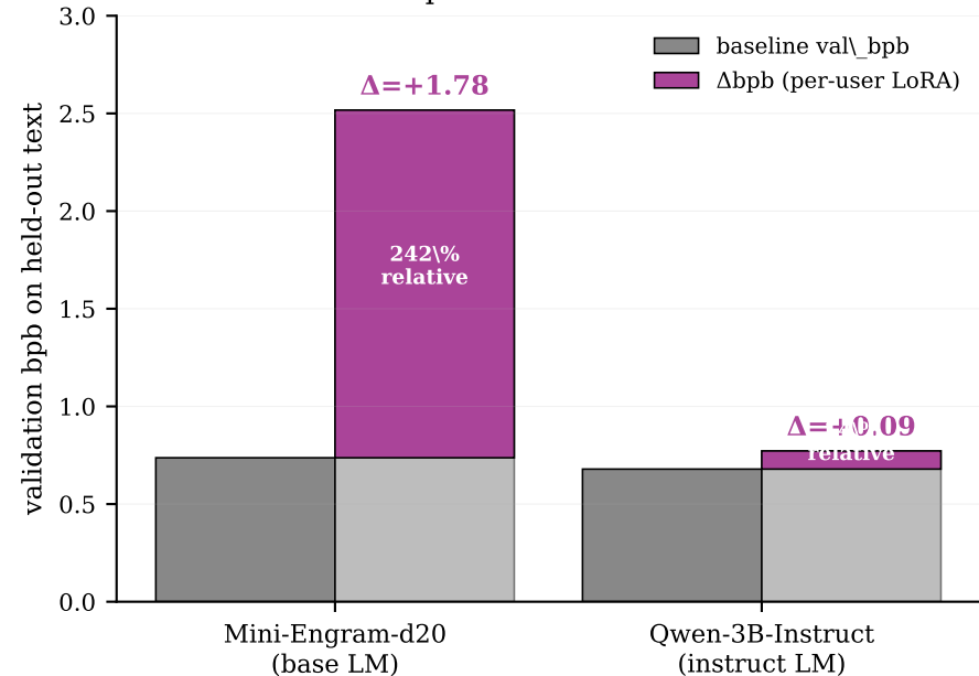
(a) Per-user LoRA contamination is present cross-base
