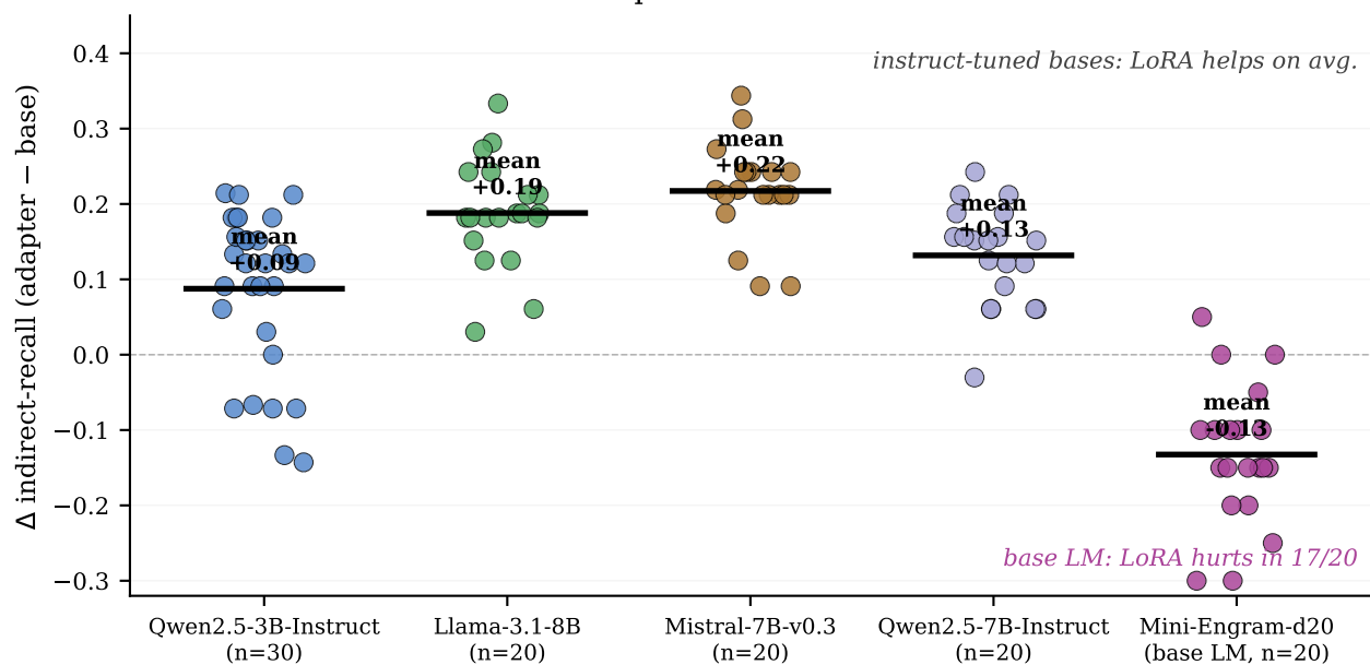
(b) Per-user LoRA's user-level effect depends on the base
