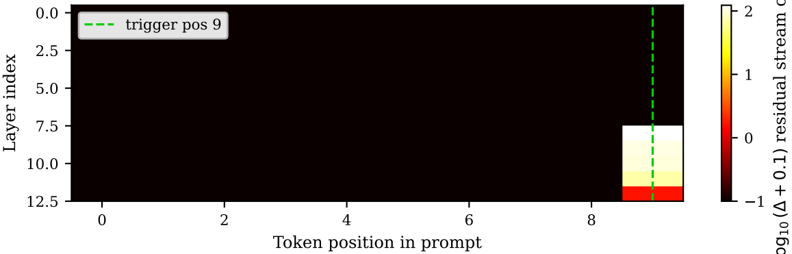
Figure 2: Engram surgical insertion is spatially perfect. \Delta = 0 at every non-trigger position, every layer.
